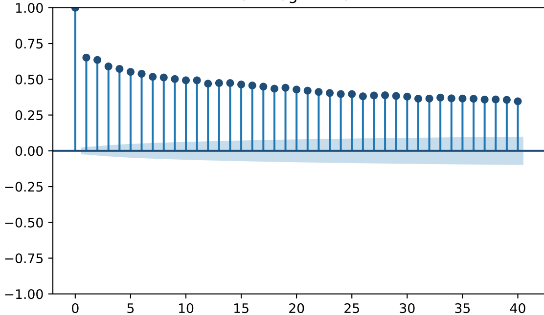
SPX log-RV ACF
