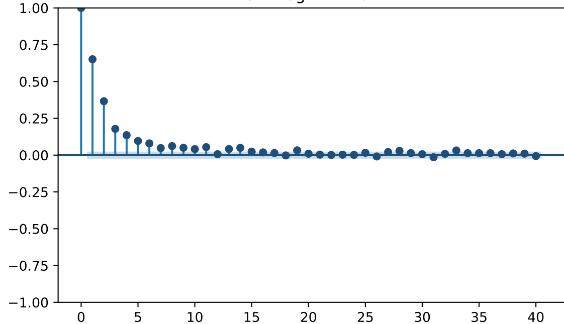
SPX log-RV PACF
