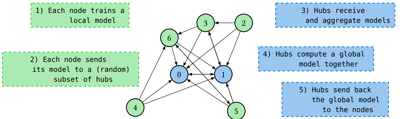
Figure 68: HEAL learning protocol: the five phases
