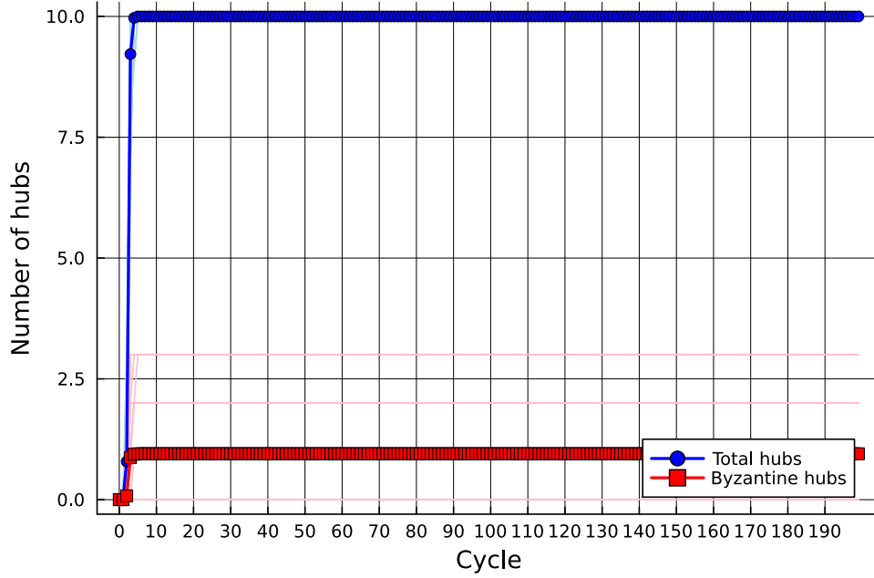
Figure 34: Independent Byzantine attack at 5% rate.
