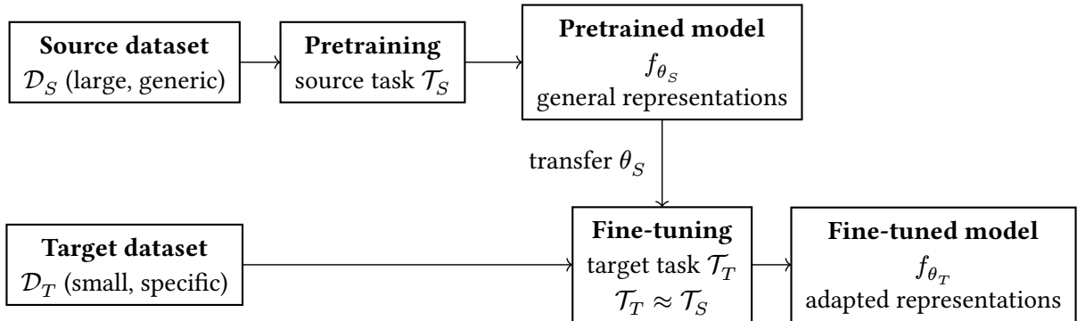
Figure 118: Transfer learning: a model f_{\theta_S} is first pretrained on a large source dataset \mathcal{D}_S for a source task \mathcal{T}_S . Its parameters \theta_S are then transferred to a fine-tuning stage on a smaller target dataset \mathcal{D}_T , yielding an adapted model f_{\theta_T} suited to the target task \mathcal{T}_T . Transfer is effective when \mathcal{T}_S and \mathcal{T}_T share underlying structure.
