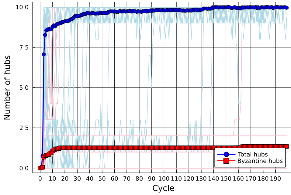
Figure 35: Byzantine hub infiltration at 1% rate.
