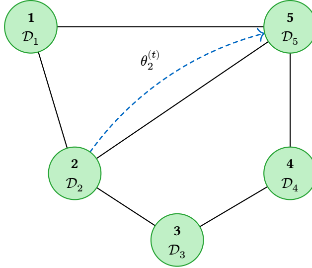
Figure 62: Gossip learning: nodes are connected in a random peer-to-peer overlay. At each round, a node selects a neighbor uniformly at random and sends its current local model.
