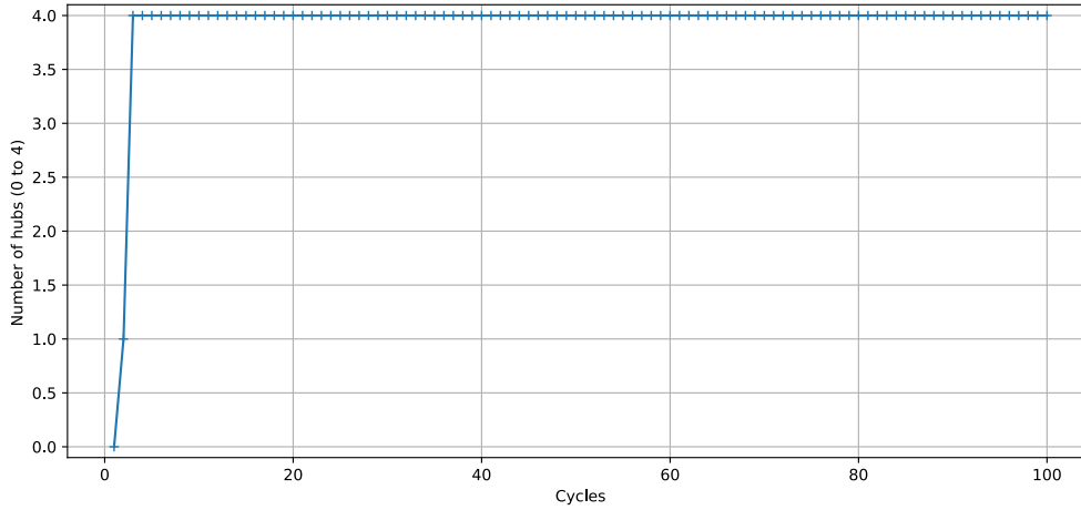
Figure 46: Number of hubs at each cycle, with N = 20 , c = 10 and h = 4
