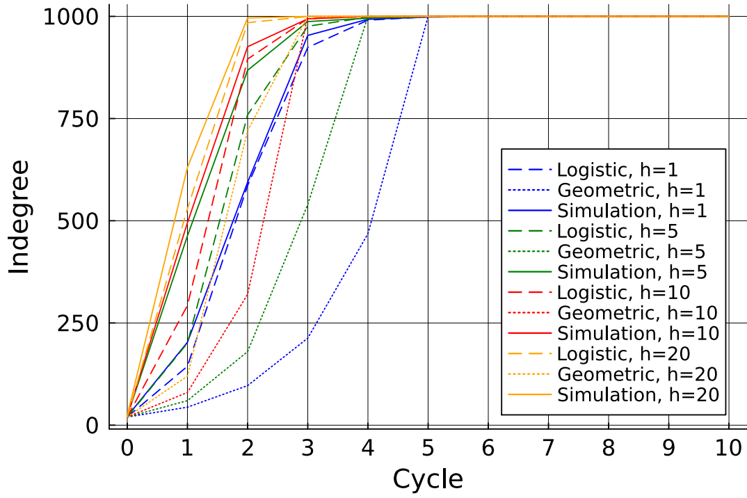
Figure 18: In-degree evolution of the hub, comparing models with simulation data, with varying values for h. K=20 , N=1000 .
