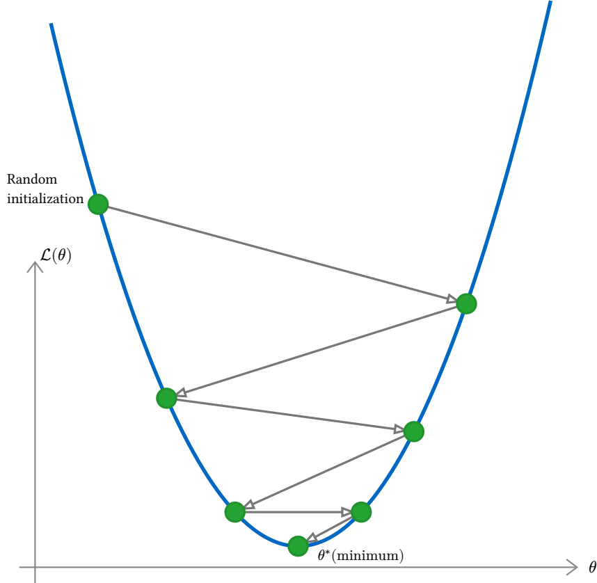
Figure 107: Gradient descent on a convex loss surface \mathcal{L}(\theta) : starting from a random initialization, the parameters \theta are iteratively updated in the direction opposite to the gradient until convergence to the minimum \theta^* .
