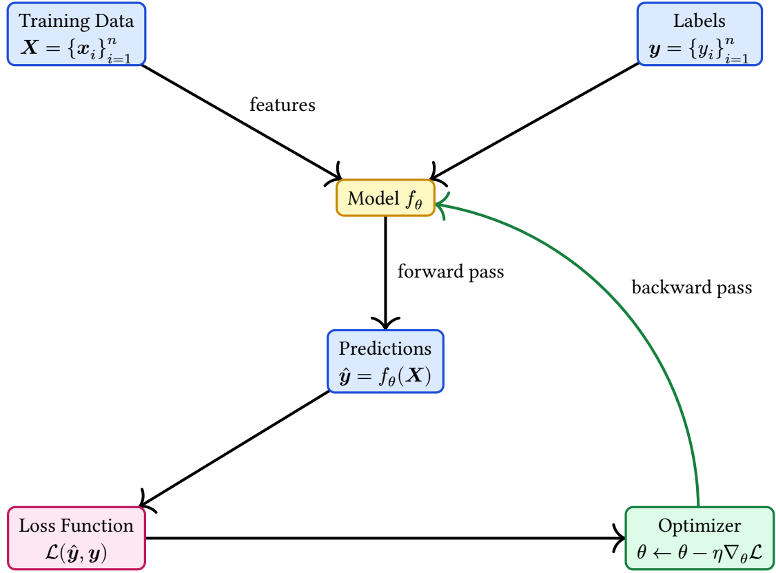
Figure 105: The supervised learning training loop.
