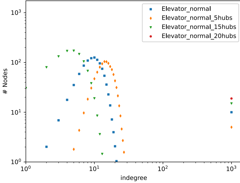
Figure 41: In-degree distribution of the network, after the run of the Elevator algorithm, with a variable number of hubs (5 hubs, 10 hubs, 15 hubs, 20 hubs). no failures.
