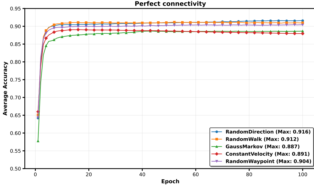
Figure 87: Accuracy evolution of FLAIR under five mobility patterns with perfect connectivity.
