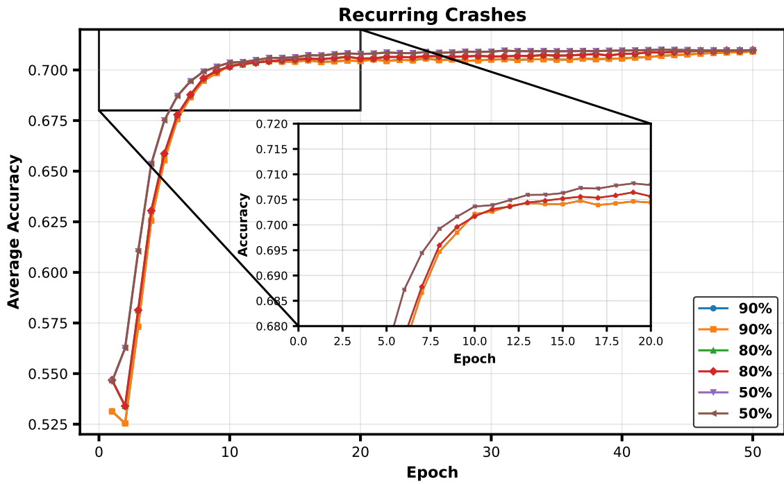
Figure 91: Accuracy evolution of FLAIR under recurring fault conditions in the smart farming scenario.
