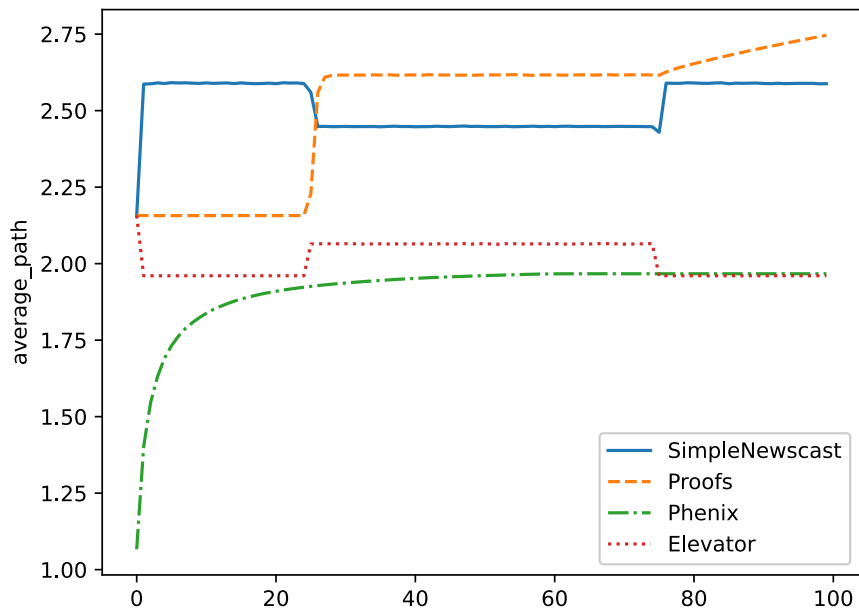
Figure 26: Average path length computed with churn, for each algorithm, every 10 cycles
