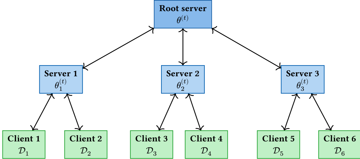
Figure 60: Hierarchical federated learning: a root server coordinates three intermediate servers, each aggregating updates from two local clients. Aggregated models propagate upward level by level until a global model is produced at the root.
