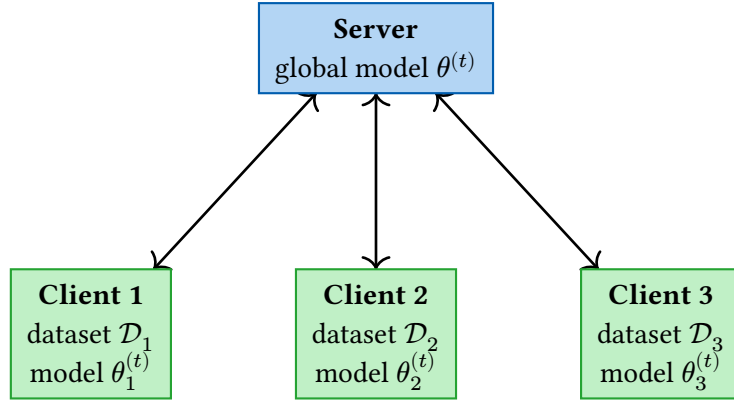
Figure 57: Federated learning with a star topology: the server broadcasts \theta^{(t)} , clients train locally on \mathcal{D}_i , and return updated parameters \theta_i^{(t+1)} for aggregation.
