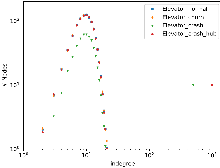
Figure 42: In-degree distribution of the network, after the run of the Elevator algorithm, during each context (no failures, 50% crash, churn, and hub-targeted failure).
