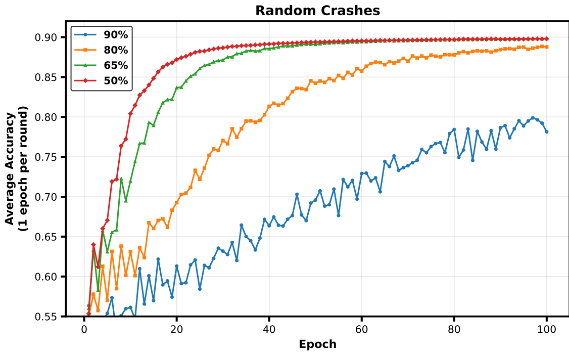
Figure 83: Accuracy evolution of FLAIR under random fault conditions (1 epoch per round).
