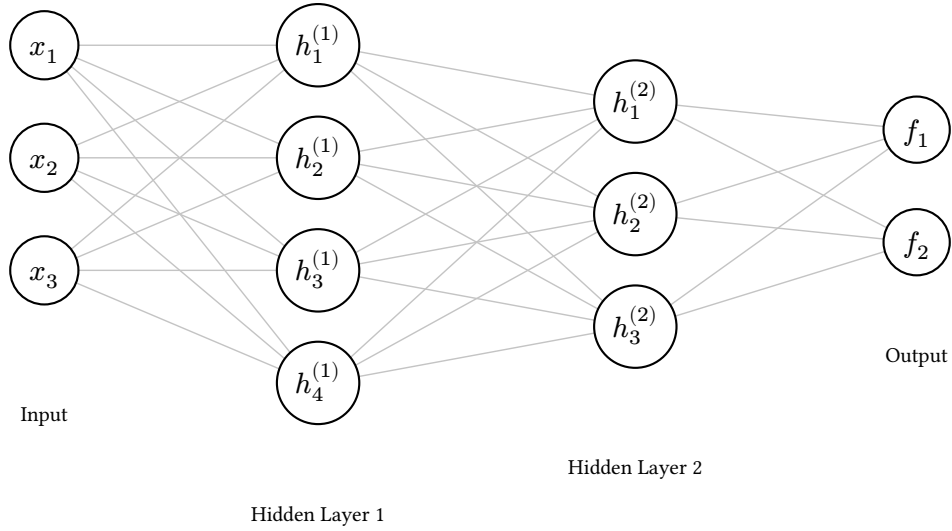
Figure 111: A fully connected neural network with two hidden layers ( L = 3 ).
