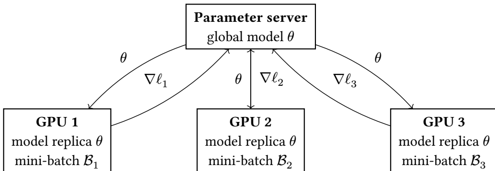
Figure 114: Data parallelism: each GPU holds a replica of the model and processes a distinct mini-batch.
