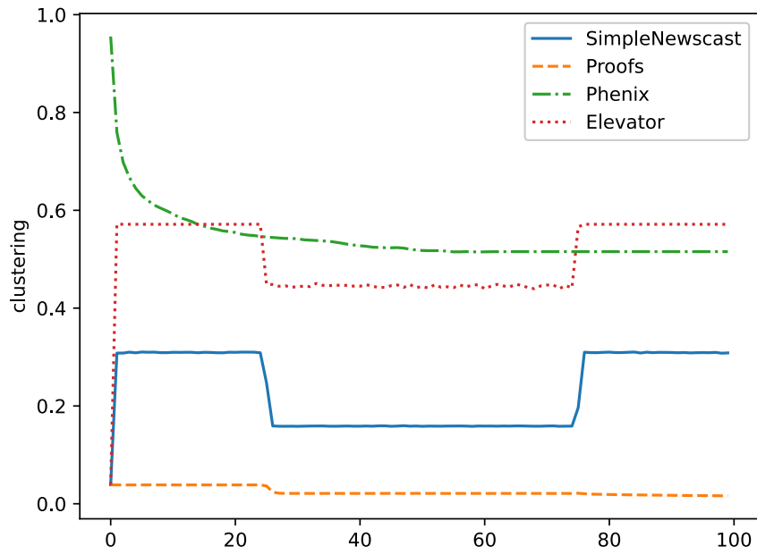
Figure 25: Clustering coefficient computed with churn, for each algorithm, every 10 cycles
