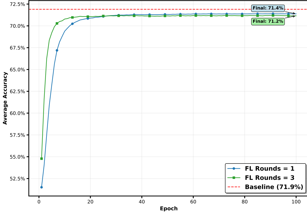
Figure 89: Accuracy evolution on the Watering the Plants dataset under the smart farming setup (80 fixed sensors + 20 mobile robots). Two local update settings ( E_{\text{round}} = 1 vs. E_{\text{round}} = 3 ) are compared against the centralized baseline (71.9%).
