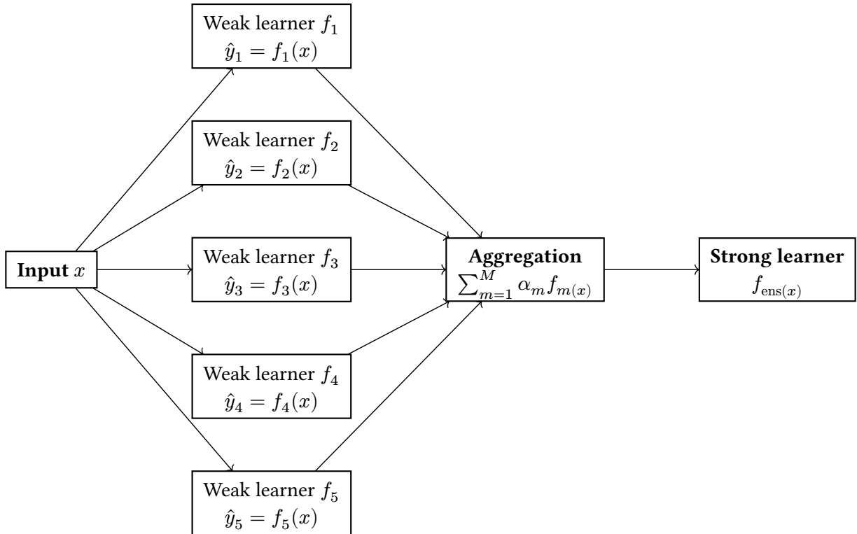
Figure 113: Ensemble learning: an input x is fed to M weak learners f_1, \dots, f_M . An aggregation step combines their predictions via a weighted sum \sum_{m=1}^M \alpha_m f_m(x)
