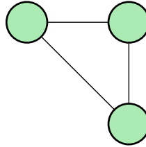
Figure 2: Example of an undirected graph with three vertices and three edges.
