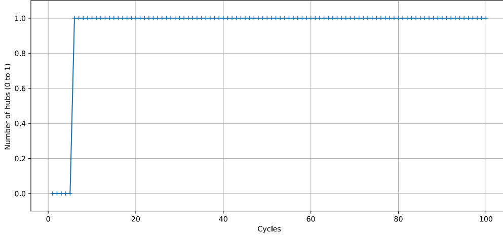
Figure 51: Number of hubs, asynchronous mode, with N = 100 , c = 20 and h = 1
