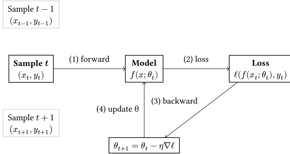
Figure 112: Online learning: the model receives one sample (x_t, y_t) at a time, computes the loss, and updates its parameters \theta before processing the next sample.
