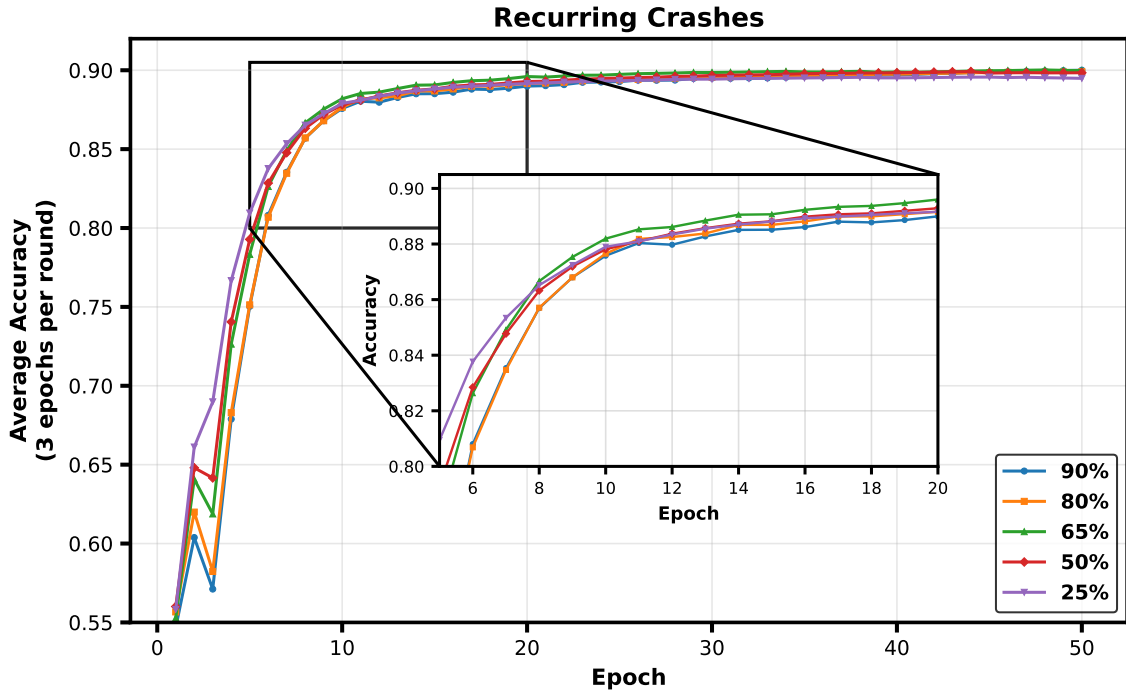
Figure 84: Accuracy evolution of FLAIR under recurring fault conditions (3 epochs per round).
