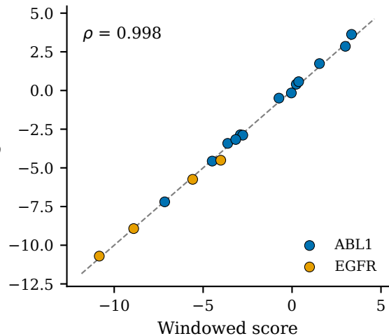
ESM-2 (150M): windowed vs. full-length
