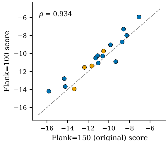
ESM-1b: flank=150 vs. flank=100
