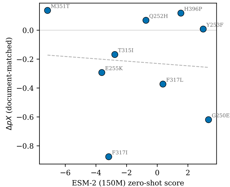
ABL1 (n=9): ESM-2 (150M) \rho=-0.167 , exact permutation p=0.678
