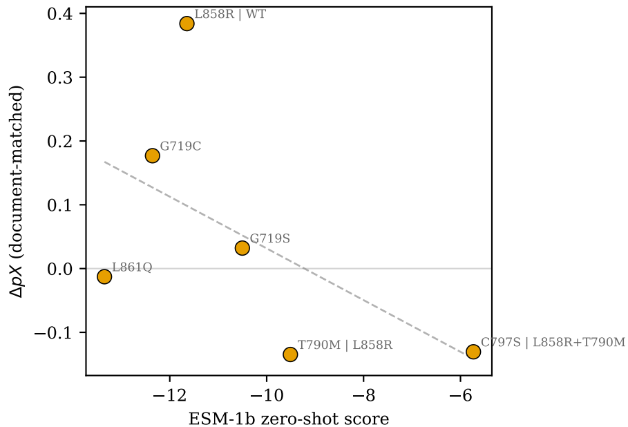
EGFR (n=6): ESM-1b \rho=-0.543 , exact permutation p=0.297
