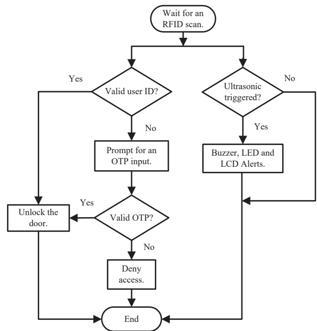
Fig.3: Functional overview of proposed system.
