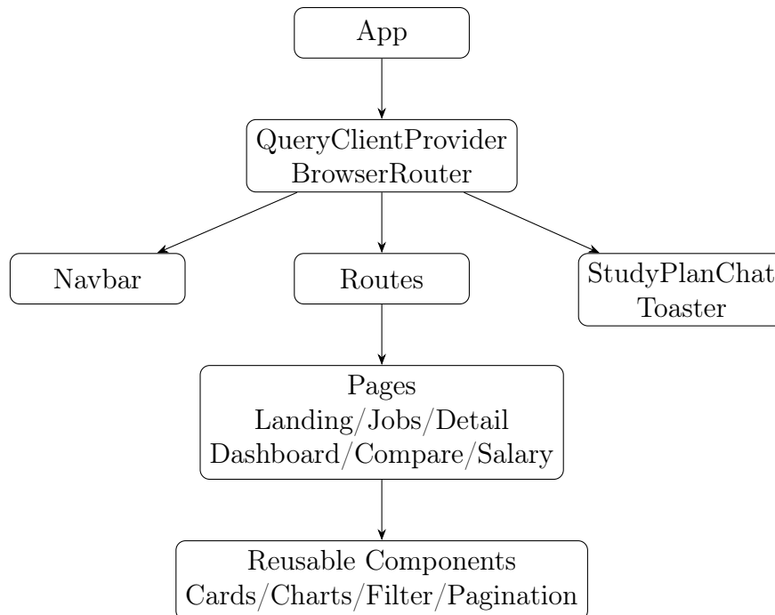
Figure 5: Frontend component hierarchy overview.
