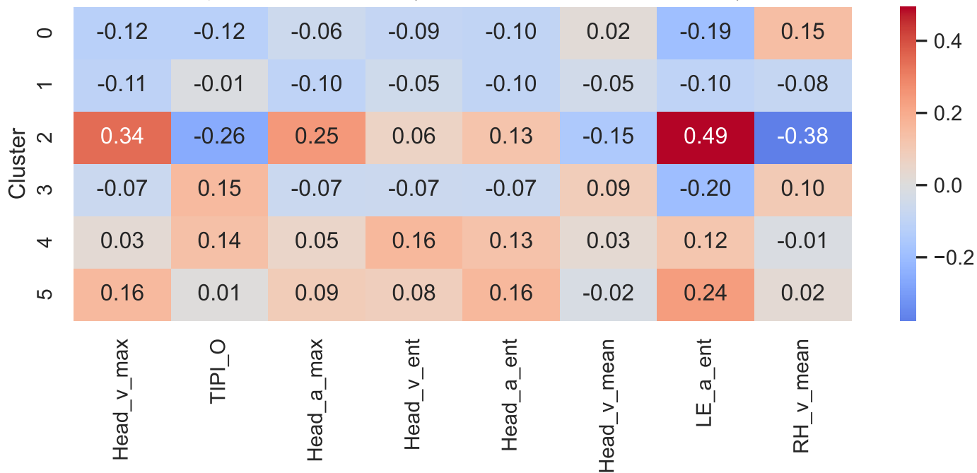
Top feature deviations (Cosine, head, acceleration, k=6)
