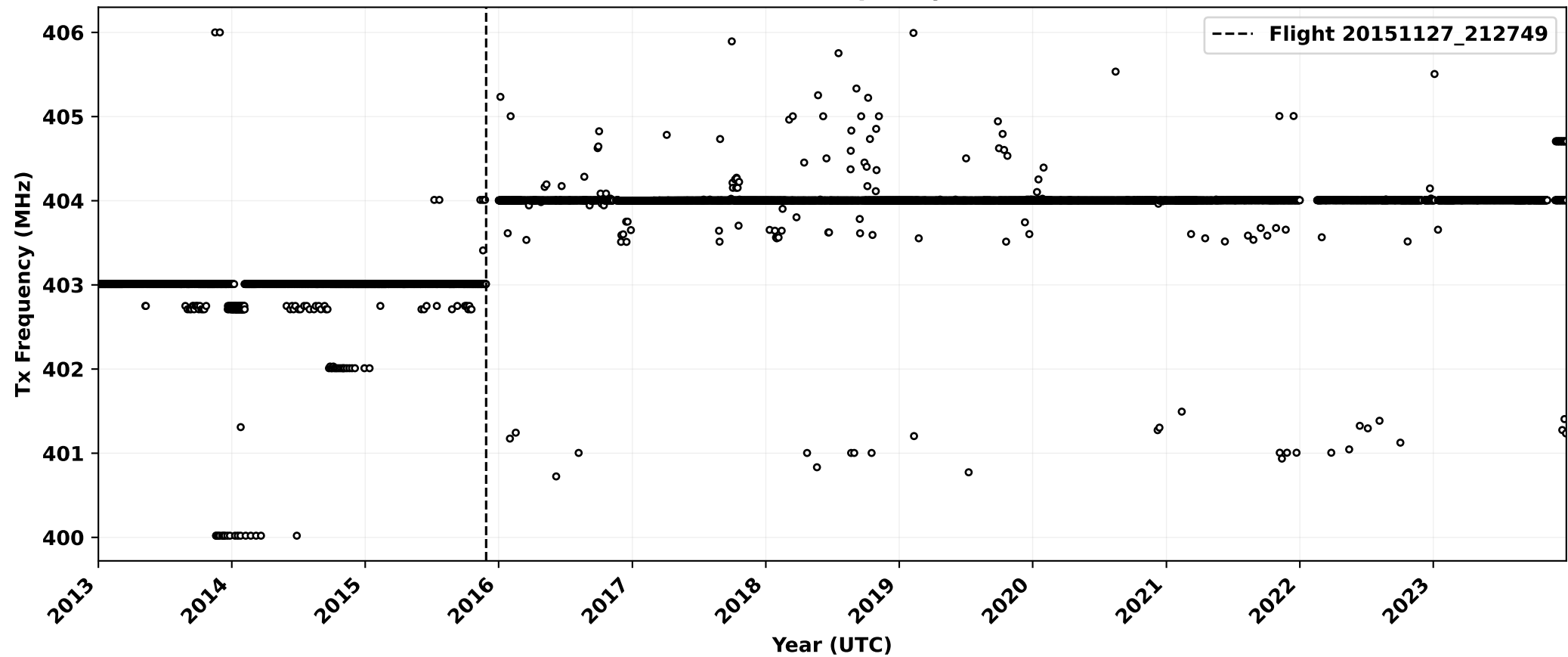
Radiosonde Transmitter Frequency Trend, 2013-2023
