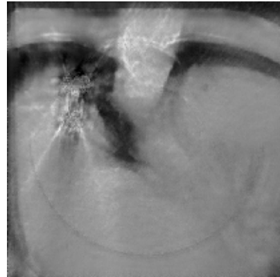
RED-CNN
