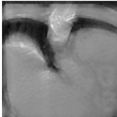
RED-CNN
