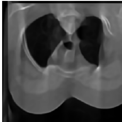
BM3D
