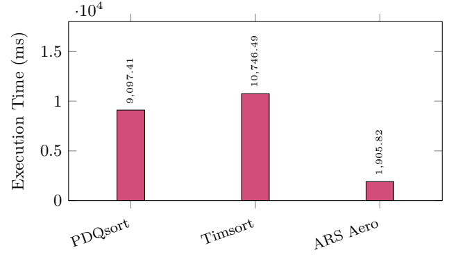
(b) Sorting 10,000,000 Random Strings
