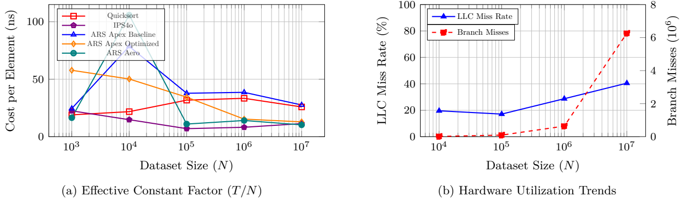
Fig. 6: Algorithmic Complexity and Hardware Utilization Scaling. As dataset size N increases, ARS constant factor stabilizes due to cache-conscious layout optimization despite scaling LLC miss rates.
