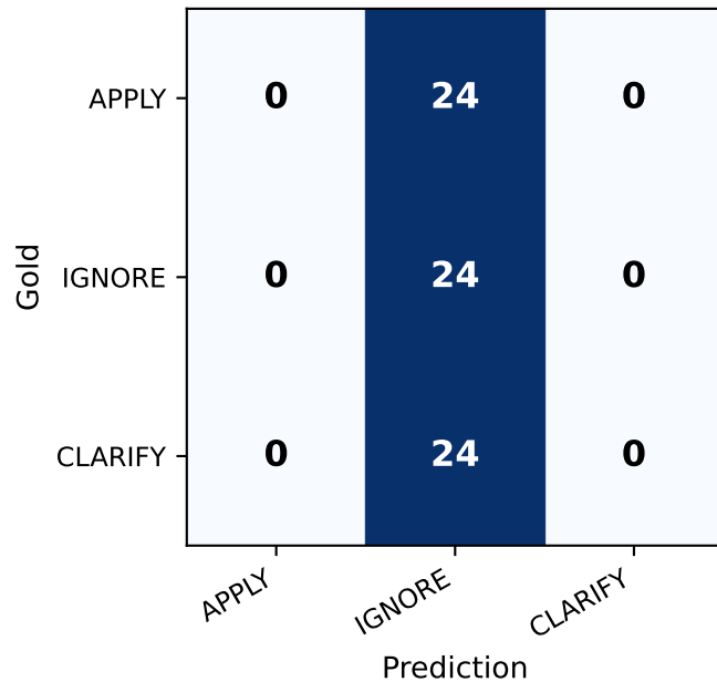
Full LLM pipeline
