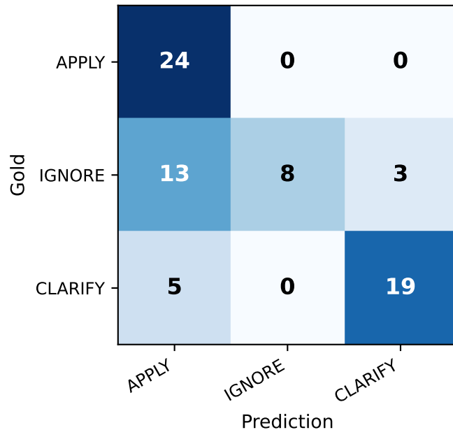
Rule memory + LLM decision
