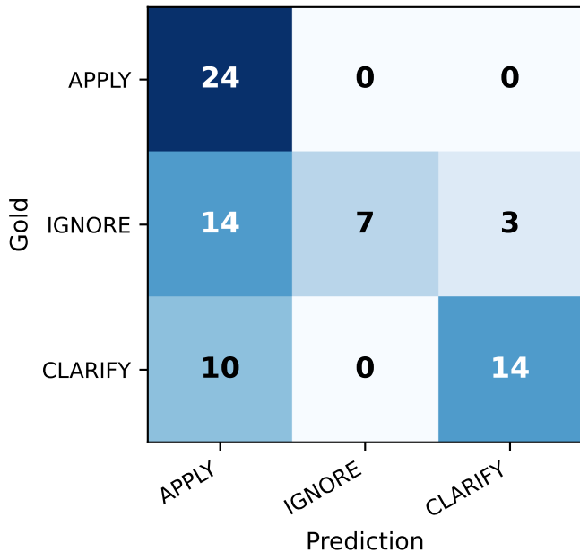
Gold memory + LLM decision
