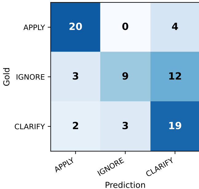
LLM memory + rule policy
