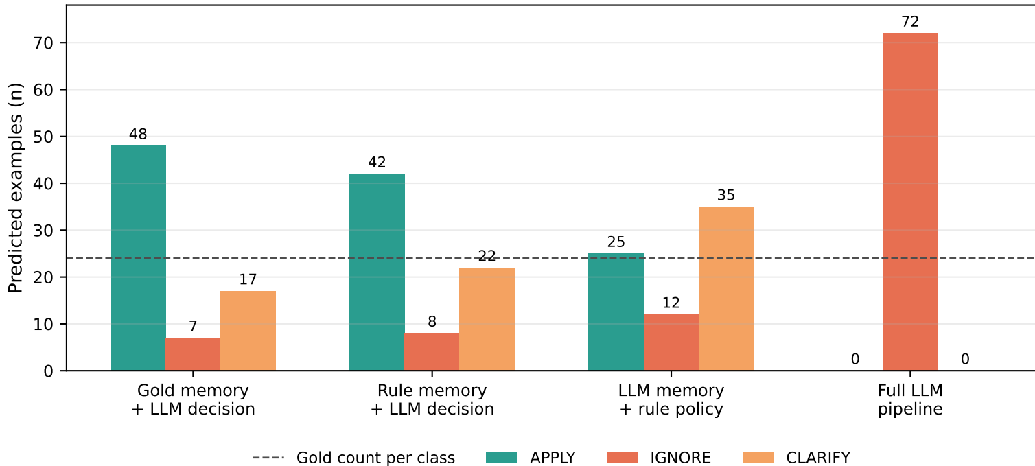
Prediction distribution (gold distribution: 24 per class)
