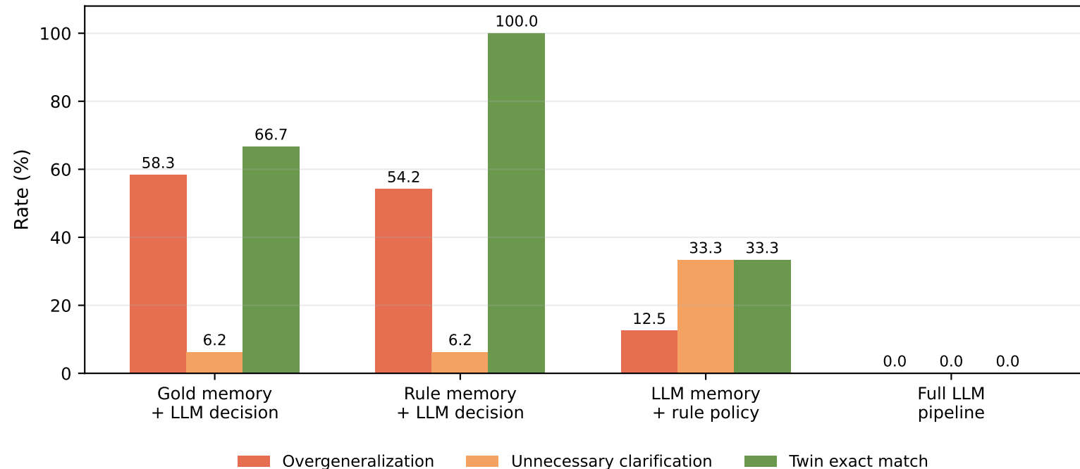
Error and counterfactual-twin metrics
