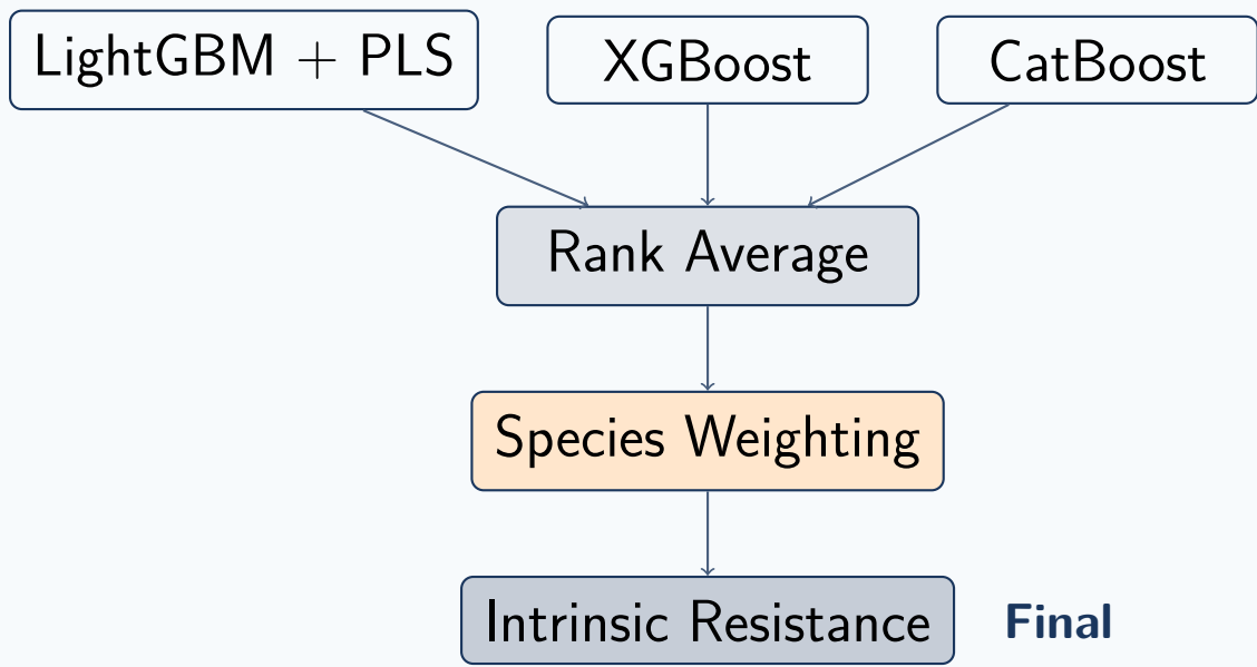
Figure 3: Final pipeline. Training: 5-fold stratified CV, LightGBM ( \text{lr}=0.02 , 350 trees, 127 leaves), PLS 100 components.
