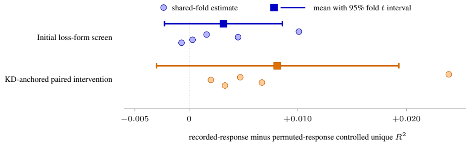
(a) Positive averaged-target trends remain uncertain at the shared-fold unit.
