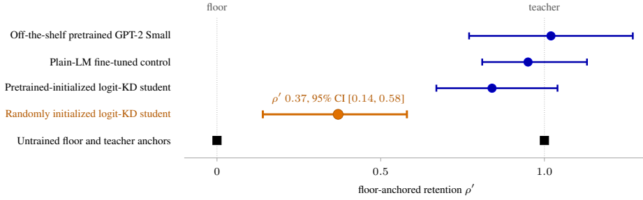
(a) Floor-anchored retention; the cold-start gap is quality-confounded and quality-aware headroom for the warm route remains unresolved.
