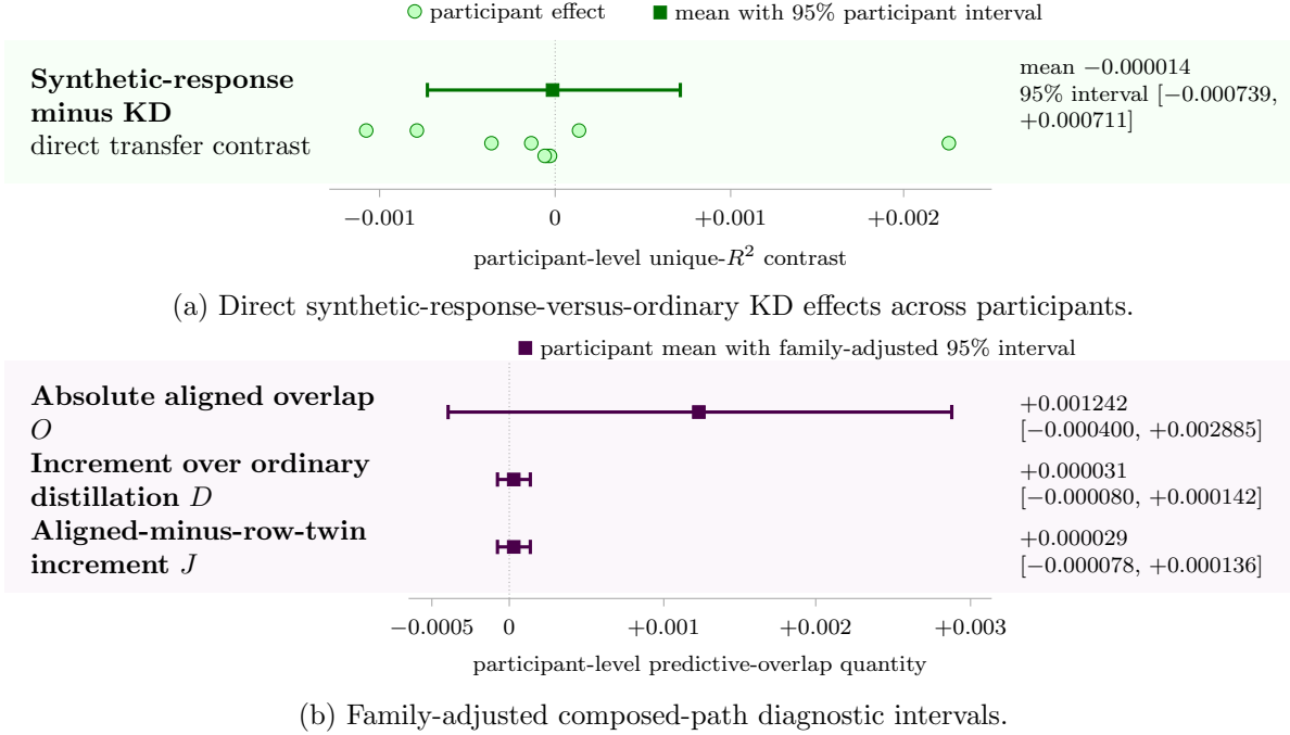
Figure 11: Direct biological transfer and the composed-path diagnostic.
