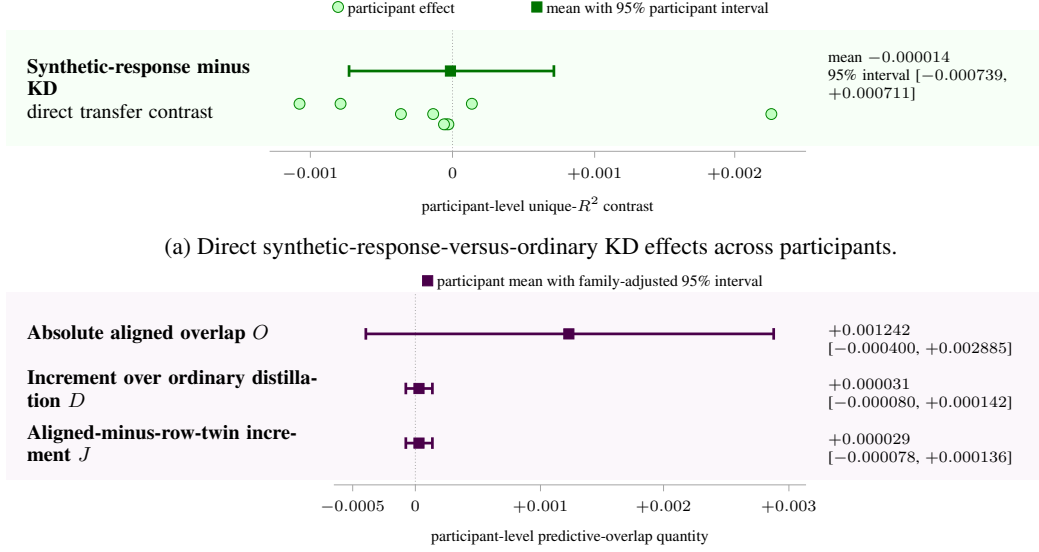
(a) Direct synthetic-response-versus-ordinary KD effects across participants. (b) Family-adjusted composed-path diagnostic intervals. Figure 11: Direct biological transfer and the composed-path diagnostic.
