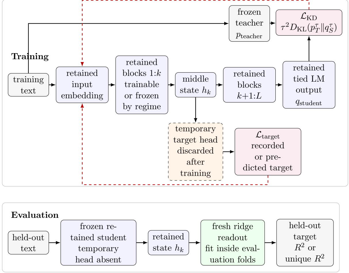
Figure 2: Training and evaluation use different heads. Solid arrows show forward computation; red dashed arrows show gradient reach. The target branch reaches the temporary head and every trainable producer of the selected state, including embeddings when they are trainable, but not later blocks through that branch. Frozen parameters receive no updates. Evaluation freezes the retained student, discards the temporary head, and fits a new ridge readout.
