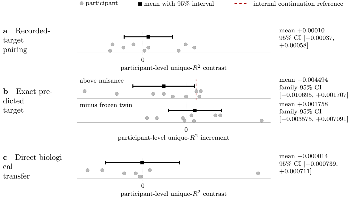
Figure 3: Participant evidence at three gates. Grey points are the same nine participants; in panel a each point is the participant median over 15 paired seed-fold cells, and the black square is the cohort mean over those nine medians. Black squares and bars otherwise show participant means and the stated 95% intervals. Panel a compares recorded-target with matched permuted-target training (+0.00010, [-0.00037, +0.00058]). Panel b uses its own scale: its top row is the exact predicted target’s increment above nuisance (-0.004494, [-0.010695, +0.001707]), and its bottom row is aligned target minus frozen row twin (+0.001758, [-0.003575, +0.007091]). Panel c compares predicted-target training with ordinary KD (-0.000014, [-0.000739, +0.000711]) on the same scale as panel a. The red line applies only to panel b’s top row; it is the inherited internal continuation reference +0.002, not an external importance threshold. All four intervals span zero; additionally, panel b’s top-row simultaneous upper end-point falls below its internal reference under the fixed assay. The intervals treat participants as the population unit after any nested seed and fold aggregation. These results localize nonpasses under the named assays; they neither prove universal nulls nor attribute a contrast to neural target content. [E008][E025][E030]
