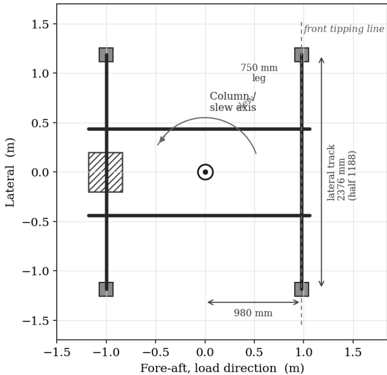
Deployed footprint with the four legs in the # arrangement. The legs stand square to the rails, so they widen the lateral track while the front line stays 980 mm ahead of the column.
