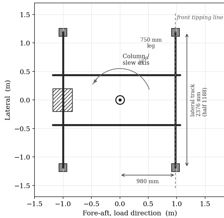
Figure 3.1 Deployed footprint in plan. The legs reach 750 mm to each side, giving a 2376 mm track, while the front foot stays on the 980 mm front line.
