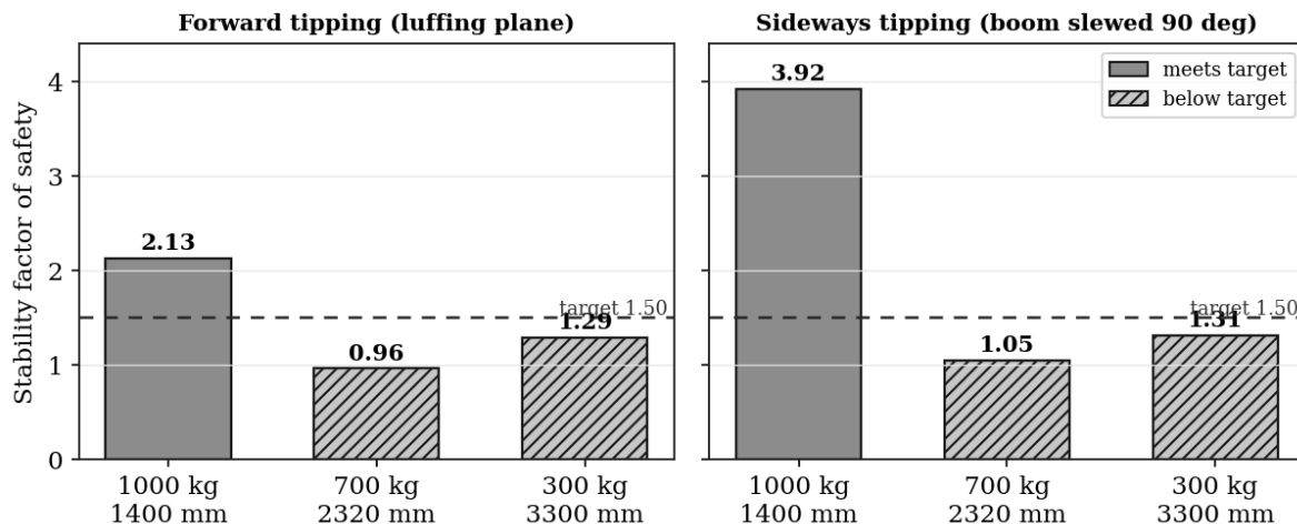
Figure 9.1 Stability in the deployed state on the corrected geometry. Forward tipping is unchanged from the wheels-only case and sits below one at mid-reach; sideways tipping clears the target only close in.
