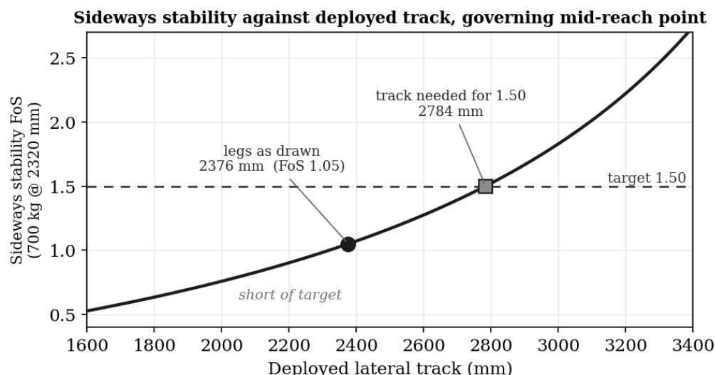
Figure 6.1 Sideways stability against the deployed track at the governing mid-reach point. The 2376 mm track from the legs sits below the 1.50 target; about 2784 mm is needed.
