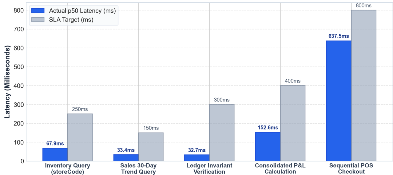
API & Database Latency Performance Benchmarks (Actual p50 vs SLA Targets)
