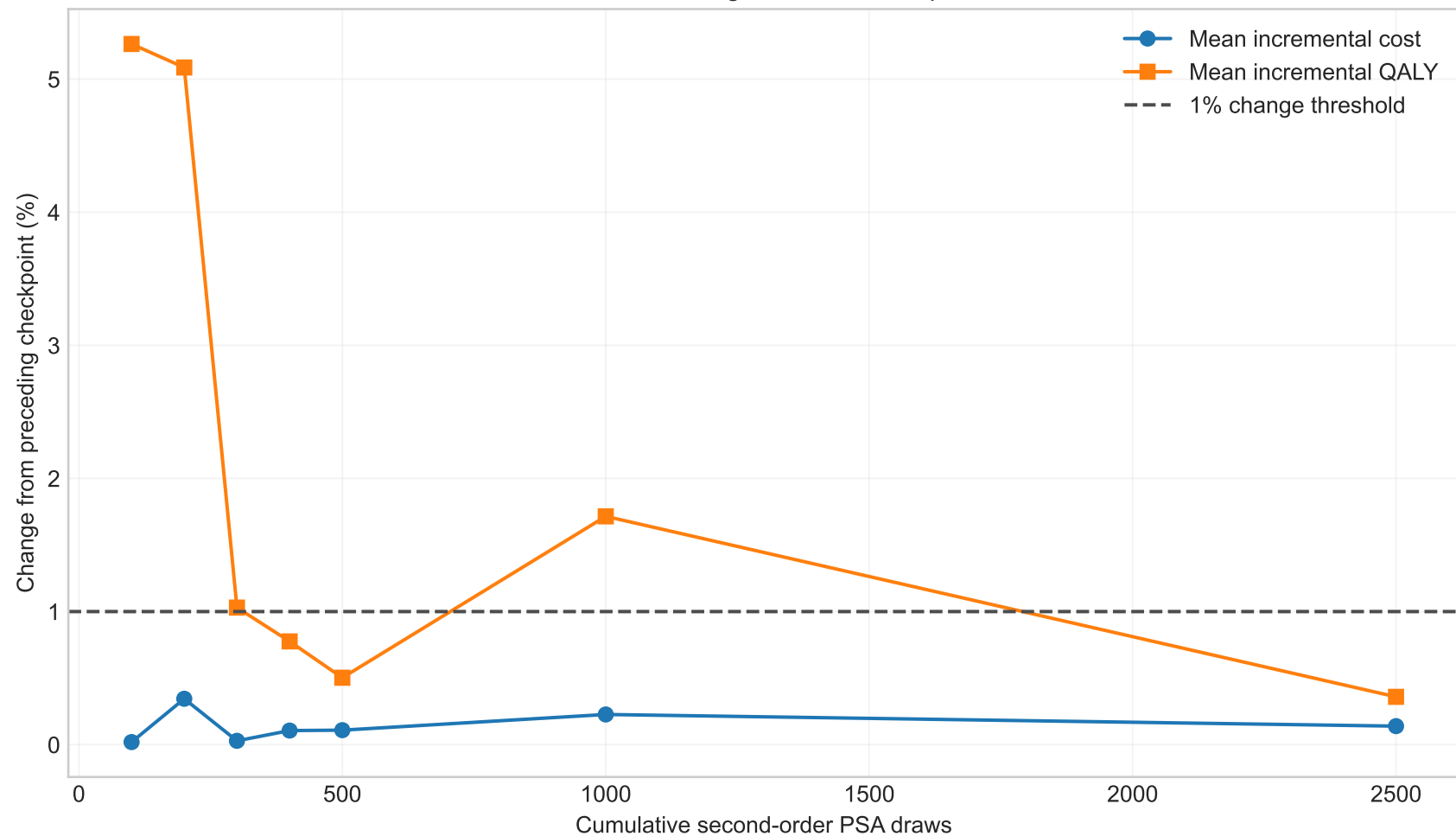
Second-order PSA convergence — FINAL production PSA
