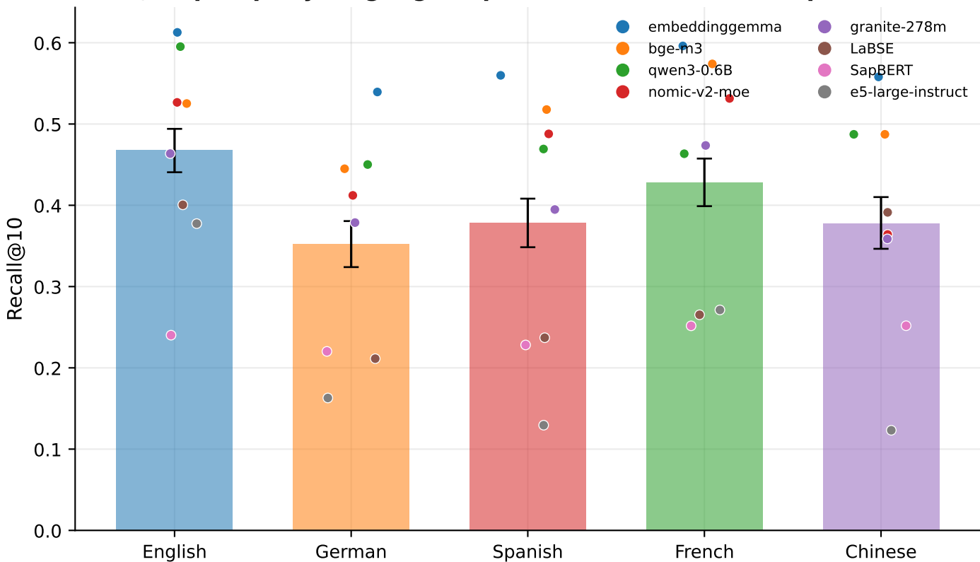
Recall@10 per query language — pooled bar (95% CI) with per-model dots
