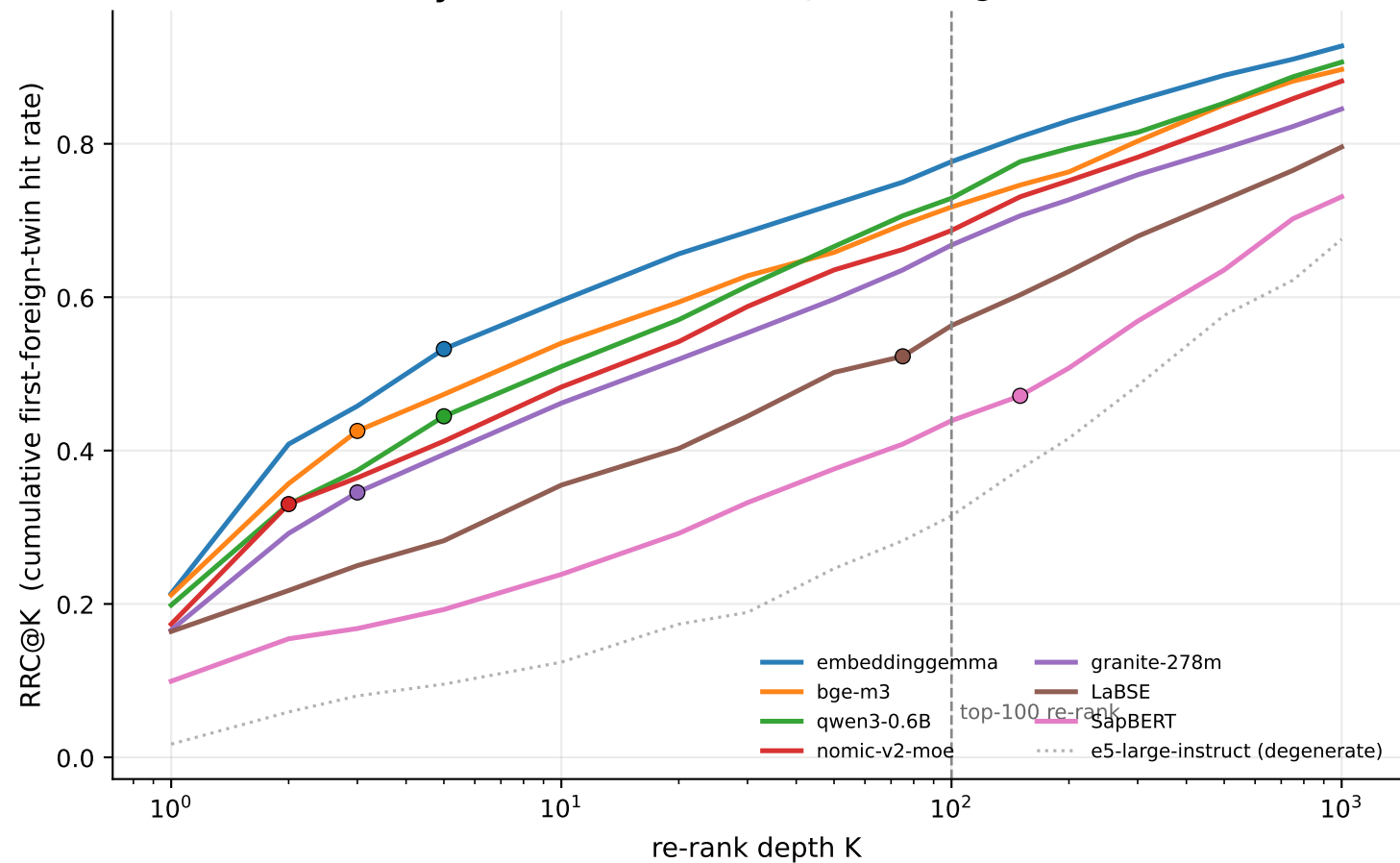
Re-ranker recoverability curves (• = knee K^* ; 1 - \text{RRC@1000} = \text{un-rerankable floor} )
