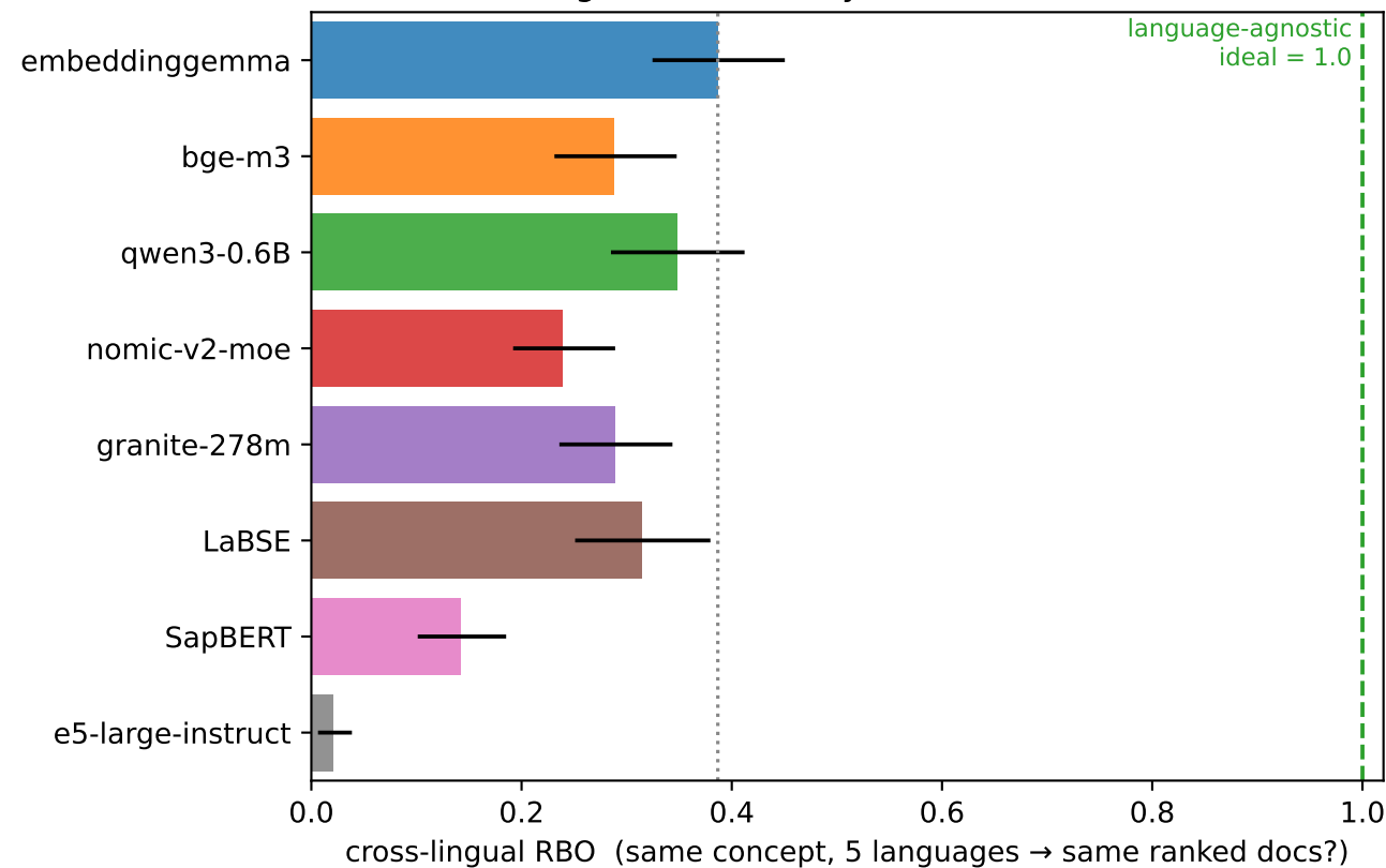
(a) Cross-lingual consistency (RBO \approx 0.39 even at best)
