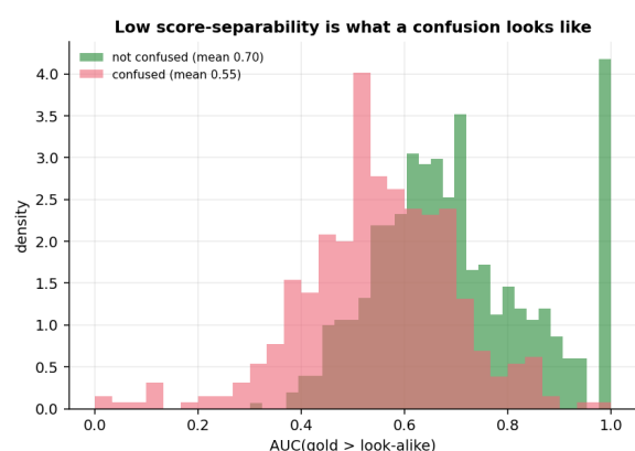
Figure 12: Confusion as separability collapse. Confused examples have weaker embedding separation between gold and non-gold documents.
