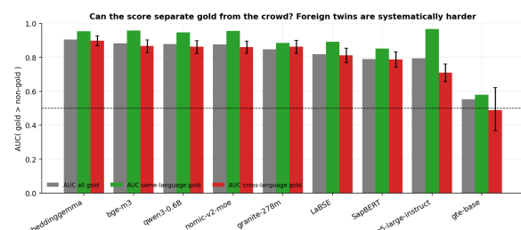
Figure 8: Embedding separability for same-language and cross-language gold documents. Lower cross-language separability indicates that the retrieval failure is partly representation-level, not only a top- k ranking artifact.
