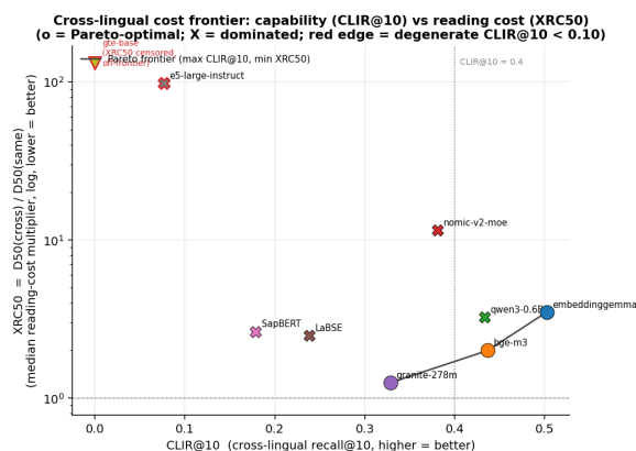
Figure 15: Cost-vs-capability view of cross-lingual retrieval. This analysis is useful for deployment decisions, but is secondary to the short paper’s core benchmark-construction story.
