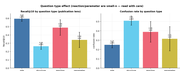
Figure 11: Question-type effects in the alias-graph benchmark. Some query types are substantially more vulnerable to chemistry-confusability than others.
