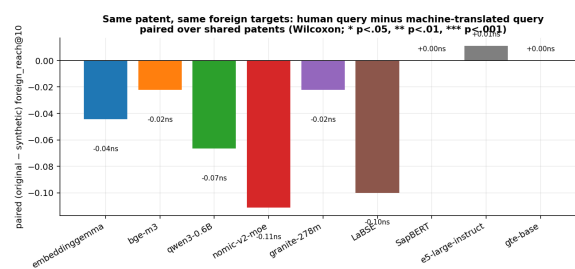
Figure 14: Human-written versus machine-translated queries. This supports the paper’s practical separation between generating query variants and relying on human-translated source evidence.
