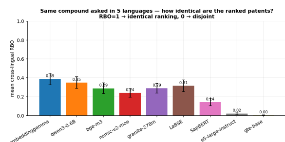
Figure 9: Cross-lingual ranking consistency for the same chemical concept asked in multiple languages. Low overlap means language variants of the same query can return substantially different ranked lists.
