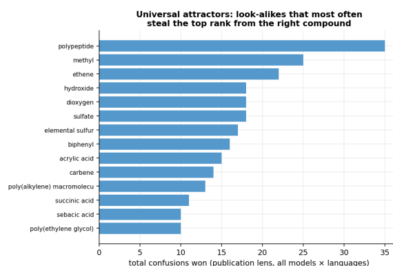
Figure 13: Universal attractors in the alias graph: chemically plausible look-alikes that repeatedly steal top rank across models or languages.
