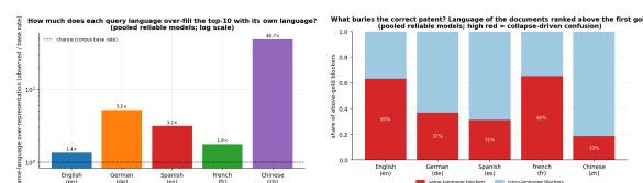
Figure 6: Language-collapse diagnostics. Same-language documents are over-represented in retrieved lists, and same-language distractors can bury cross-language gold evidence.
