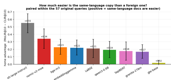
Figure 4: Same-language home advantage by model. The gap between same-language and cross-language retrieval is the main reason aggregate recall can overstate deployment readiness.
