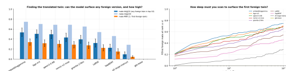
Figure 7: Foreign-twin retrieval diagnostics. The figure reports whether multilingual publication variants are found and how deeply a model must search before reaching the first cross-language twin.
