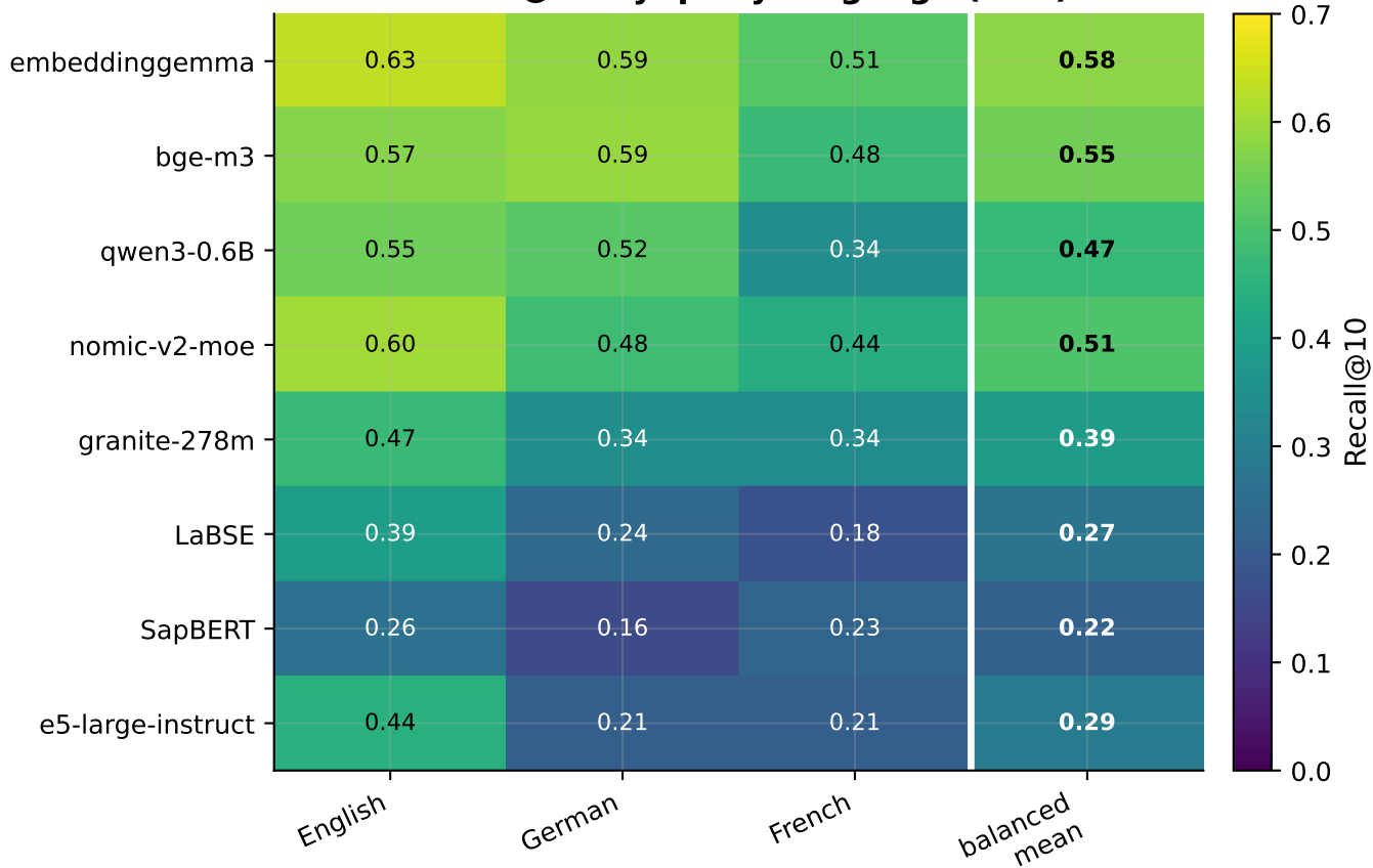
Recall@10 by query language (EPO)
