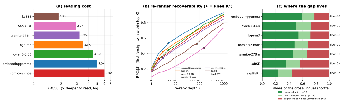
Figure 6: Deployment cost of cross-lingual retrieval. The panels separate how deep a user must read, how much a re-ranker can recover from a candidate pool, and which part of the cross-lingual shortfall remains an alignment-only failure for the first-stage retriever.
