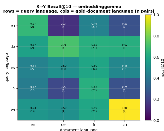
Figure 7: Directional query-language \rightarrow document-language retrieval. Cross-language retrieval is not symmetric: a model’s behavior depends on both the query language and the target document language.
