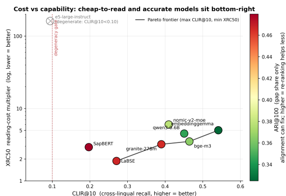
Figure 7: Deployment-oriented cost-vs-capability frontier. Cross-language Recall@10 measures capability, while XRC50 measures how much deeper a user must read to reach cross-language evidence. The frontier makes the capability/cost trade-off explicit rather than choosing a model from aggregate recall alone.
