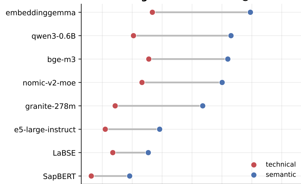
Google Patents — Hit@10
