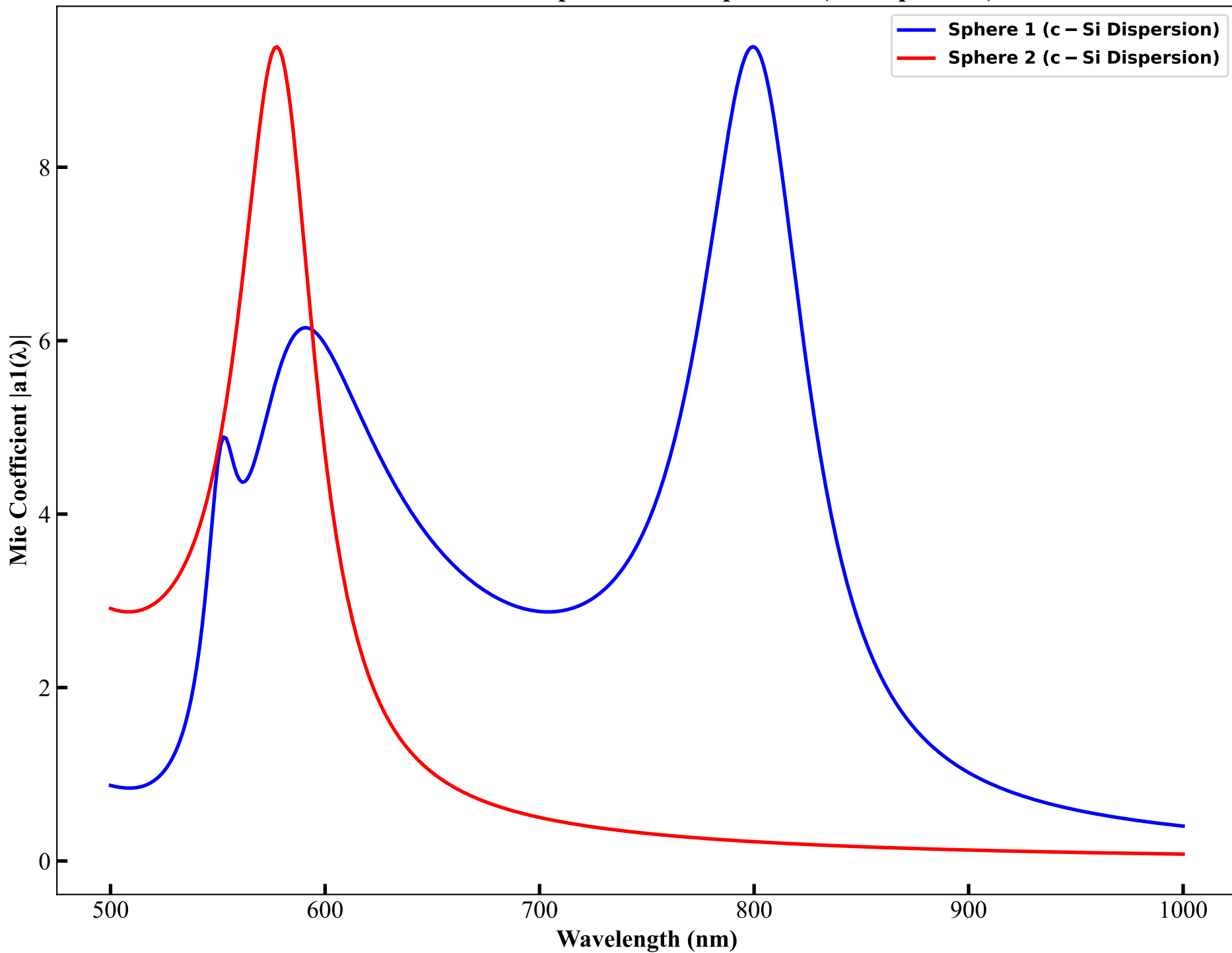
Mie Coefficients for Sphere 1 and Sphere 2 (Si Dispersion)
