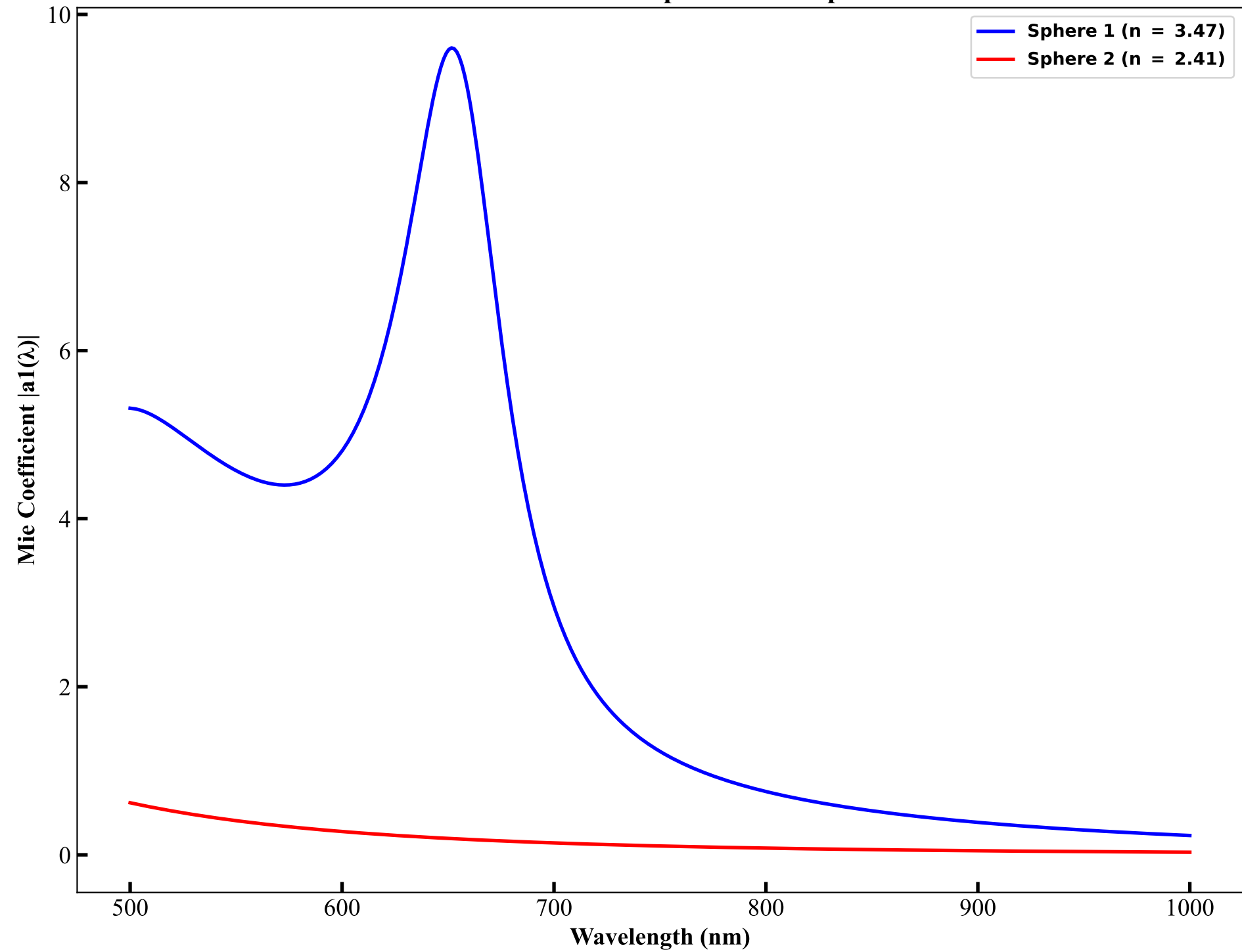
Mie Coefficients for Sphere 1 and Sphere 2
