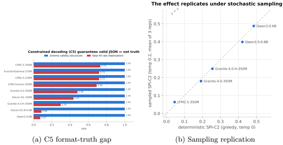
Fig. 2. (a) C5 constrained decoding gives parseable, schema-valid JSON for every compatible model, but field level correctness varies widely. (b) The five models with positive deterministic SPI-C2 remain positive at temperature 0.2 across three repetitions.
