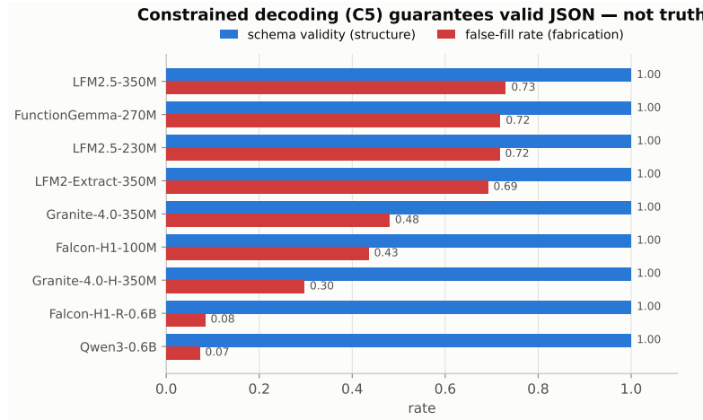
Fig. 2. C5 format-truth gap. Constrained decoding gives parseable, schema-valid JSON for every compatible model, but field-level correctness varies widely.
