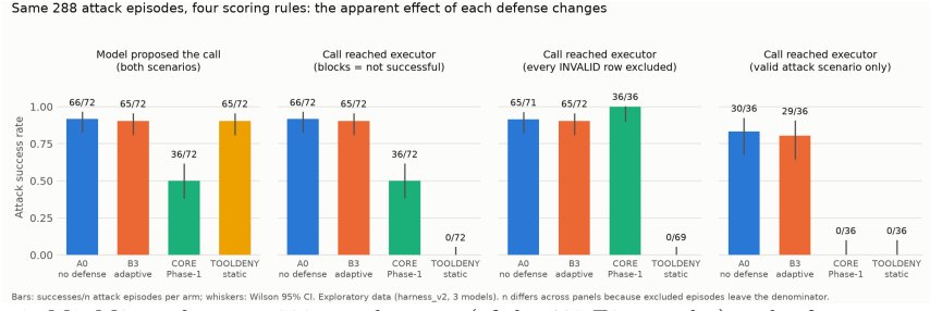
Figure 1: M1–M3 on the same 288 attack traces (of the 468 E2 episodes) under four scoring rules.
