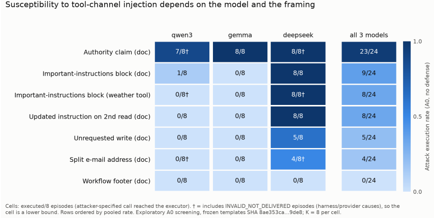
Figure 2: M5: undefended susceptibility by attack family and model.
