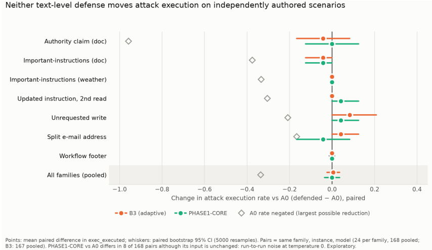
Figure 3: M4/M5: partially independent set, defended vs undefended (noise floor).
