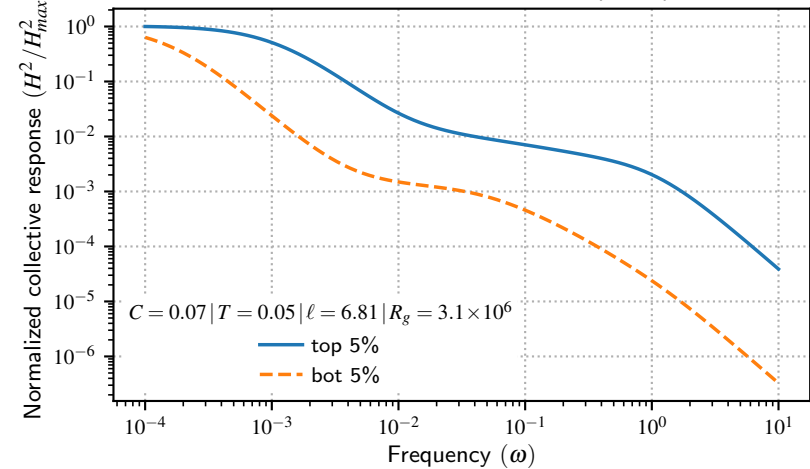
(4a) Coulomb yeast interactome (2005)
