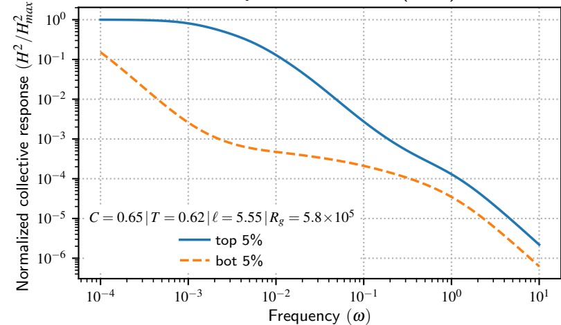
(2a) Political blogs network (2004)
