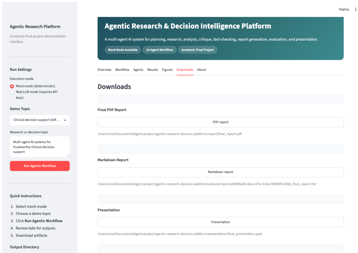
Figure 10: Actual Streamlit Downloads tab captured in a headless browser after mock demo run.
