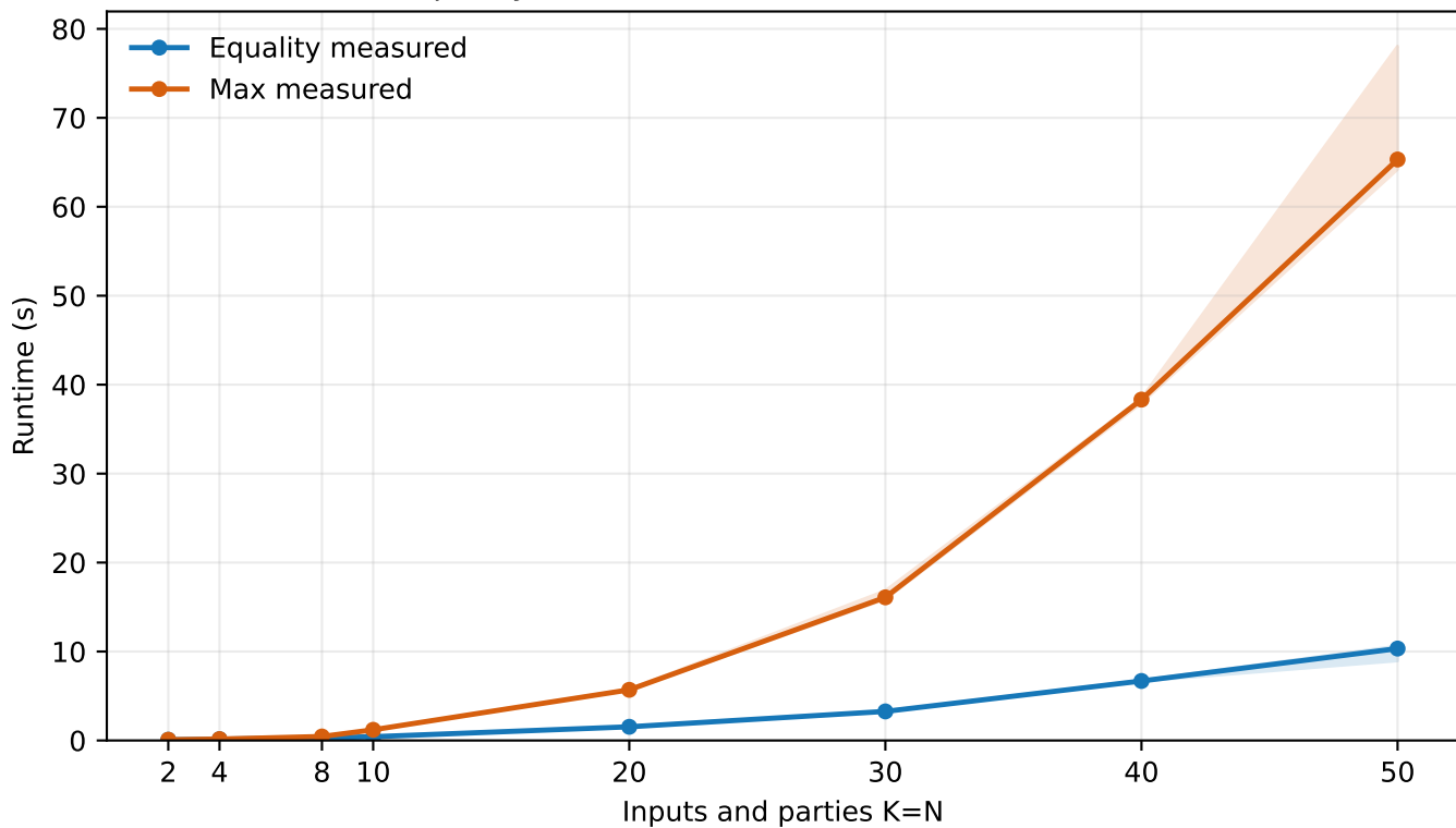
Equality and Max runtime (s) vs. N (linear axes)
