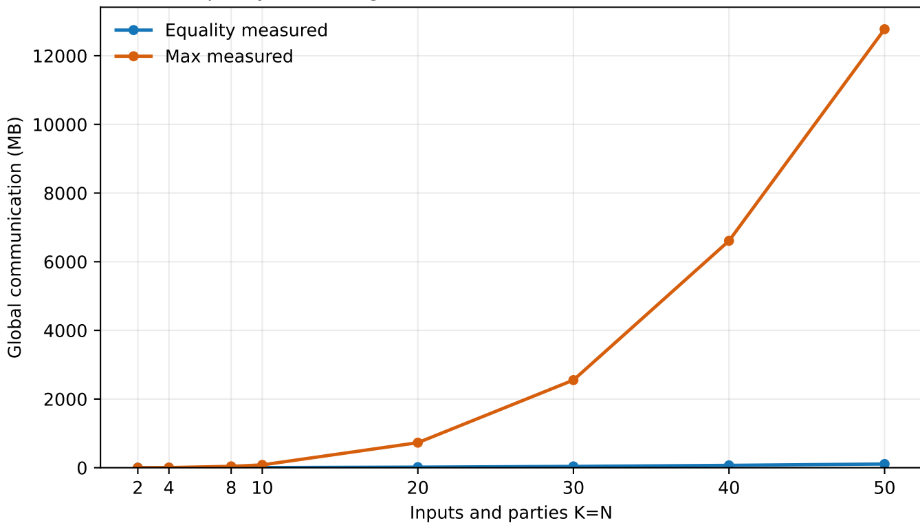
Equality and Max global communication (mb) vs. N (linear axes)
