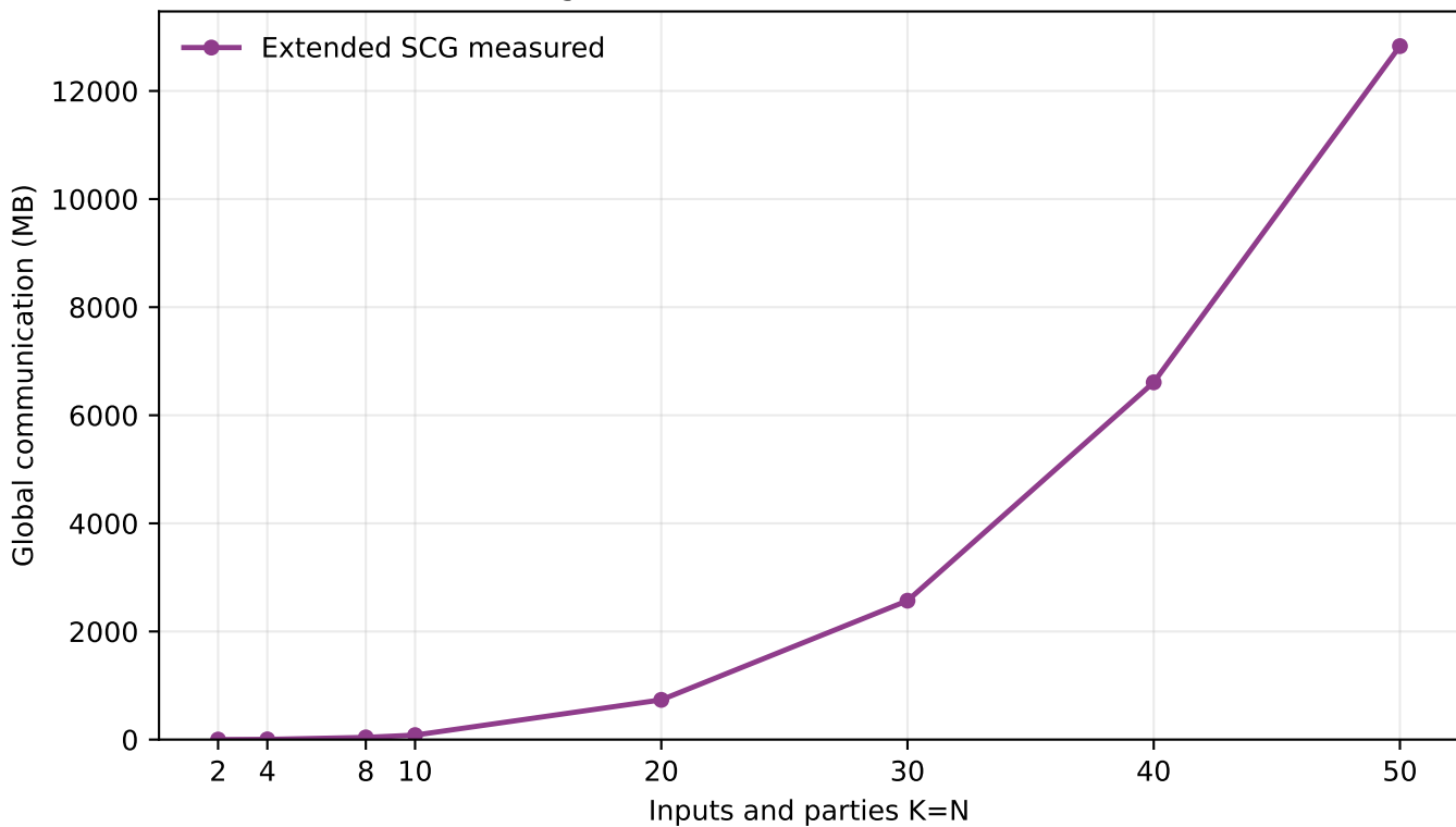
Extended SCG global communication (mb) vs. N (linear axes)
