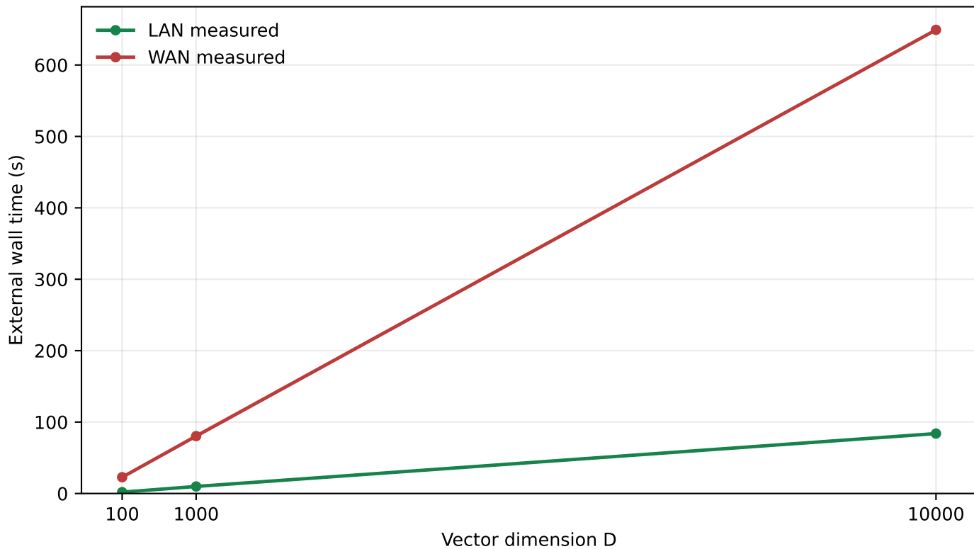
Actual tc netem LAN vs. WAN: secure Median (linear axes)
