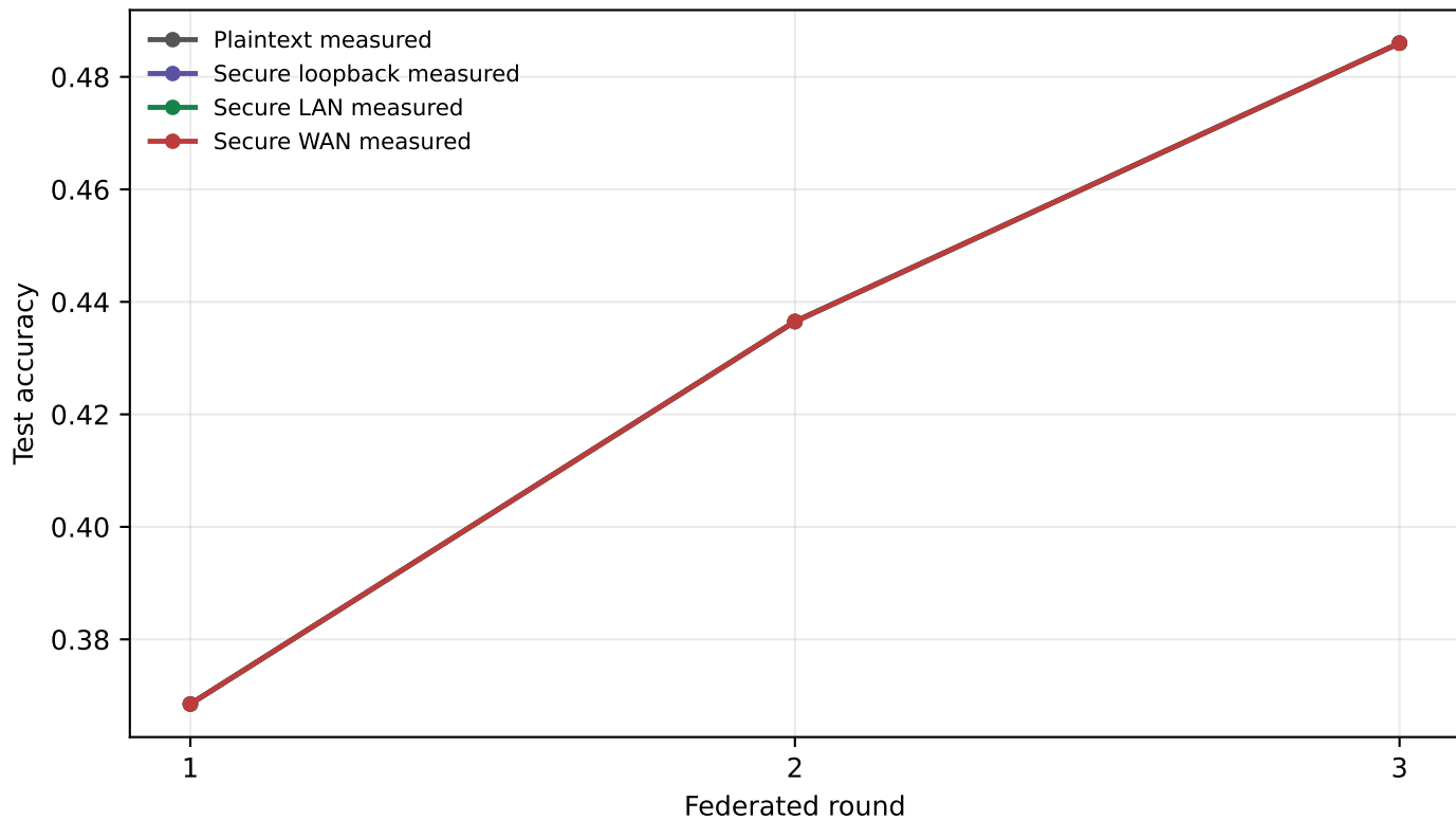
MNIST test accuracy by federated round (linear axes)
