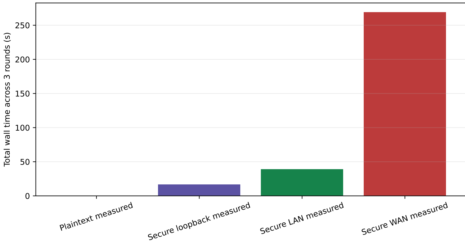
End-to-end MNIST training time comparison (linear axes)
