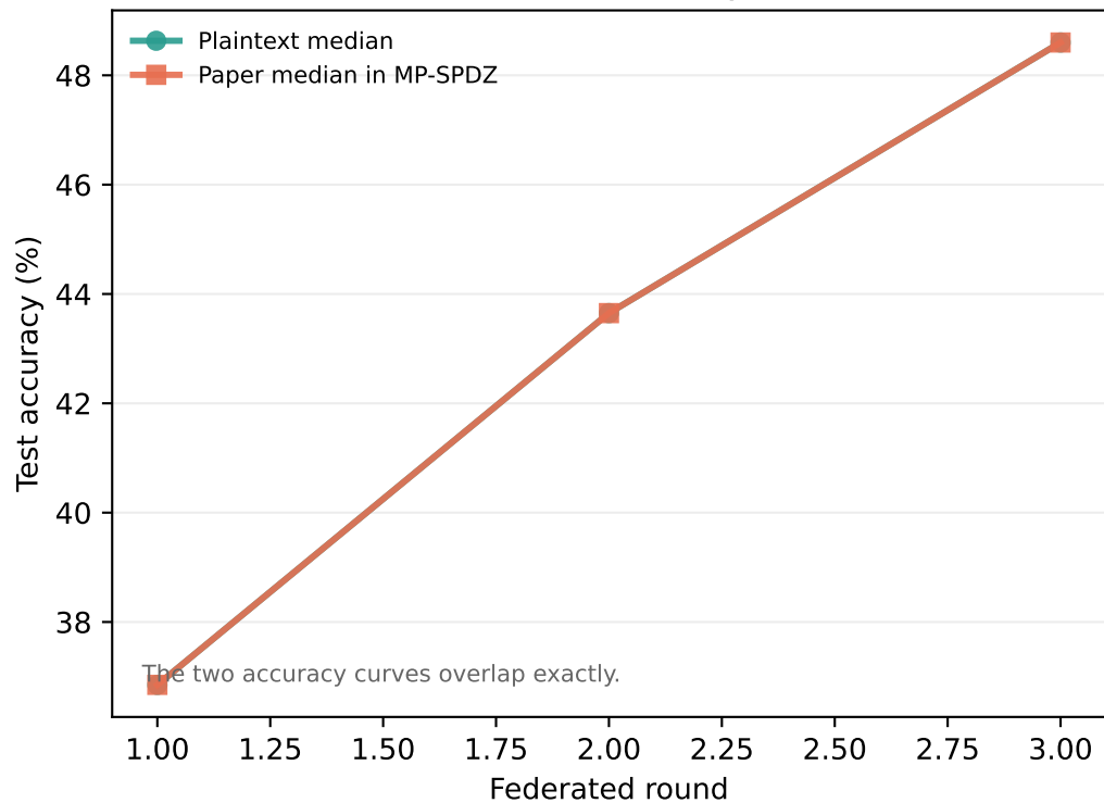
MNIST accuracy
