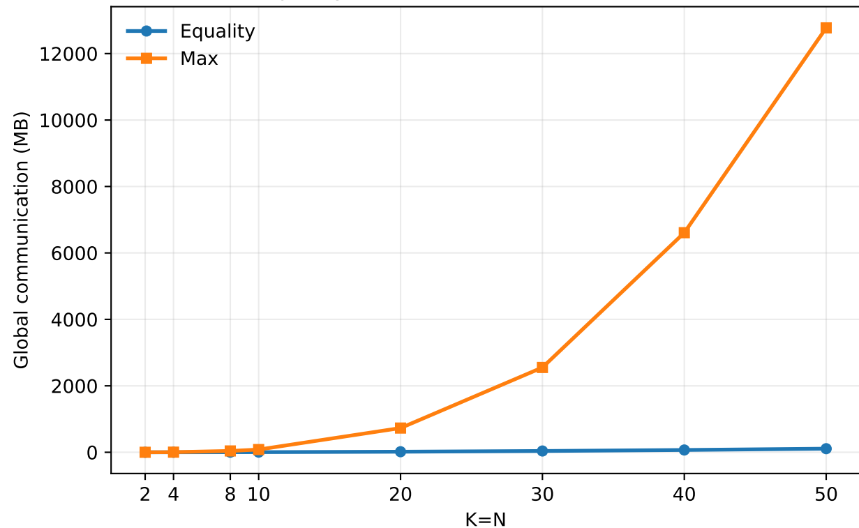
Equality and Max communication (L=32)
