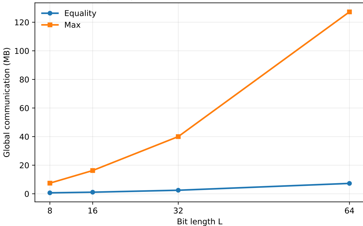
Equality and Max communication ( K=N=8 )
