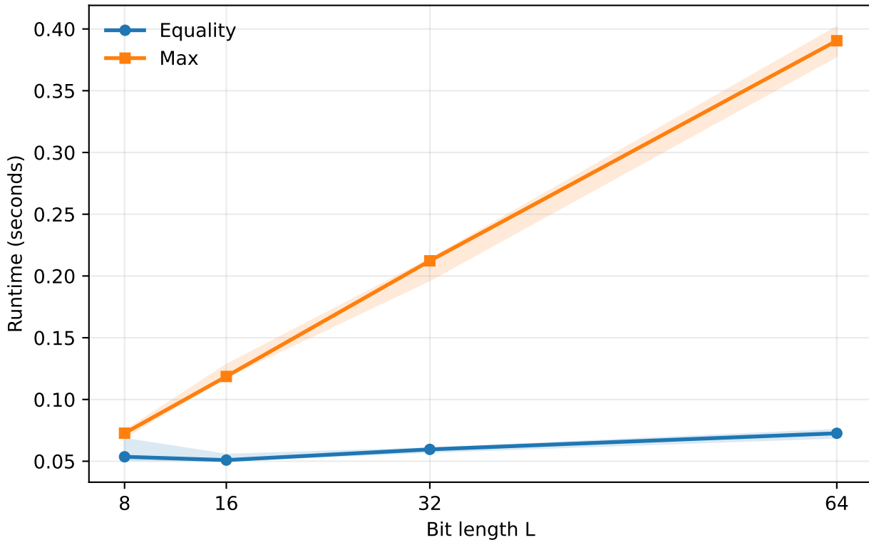
Equality and Max runtime (K=N=8)
